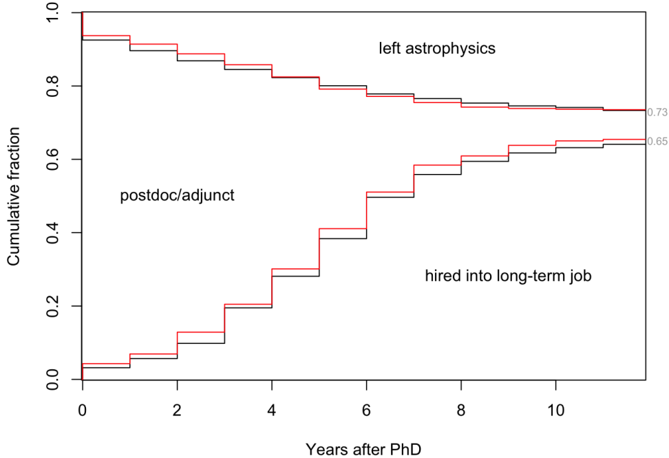
Figure 2. Career status by year after PhD for men (black) and women (red) astronomers. The middle wedge indicates the fraction still in temporary positions; the top wedge indicates astronomers who left the field while the bottom wedge indicates those who secured long-term employment. Years > 7 have been corrected for incompleteness using our hazard model.
