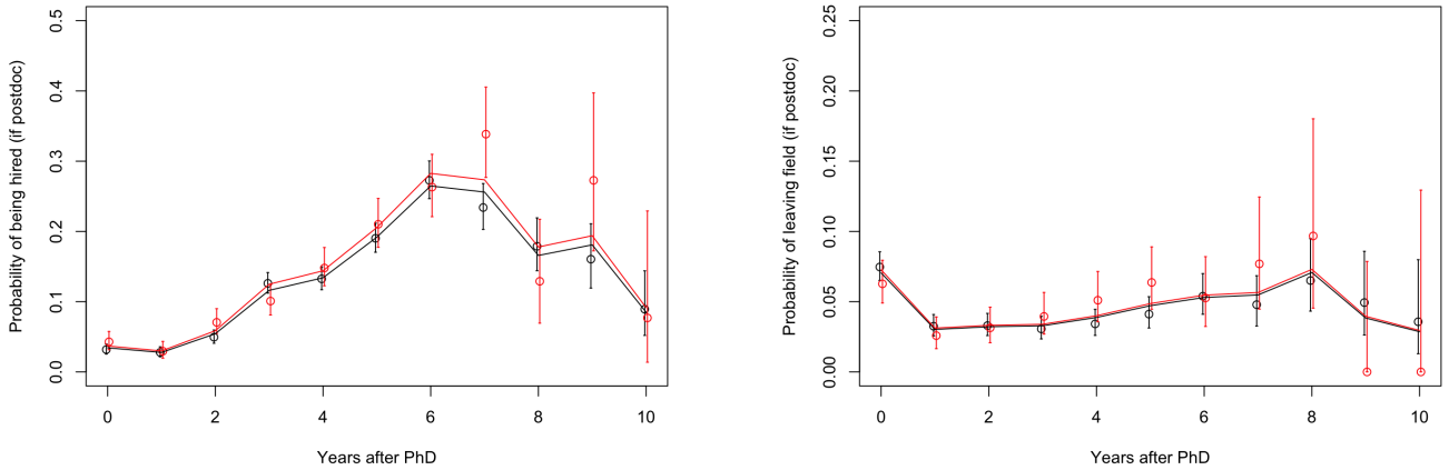
Figure 4. Hazard curves for astronomy PhDs (points), along with the best-fit proportional-hazard model (lines). This shows the probability of a postdoc/adjunct being hired into a long-term astronomy position (left) or leaving the field (right) at a given year post-PhD. Women and men are hired and leave the field at essentially identical rates.
