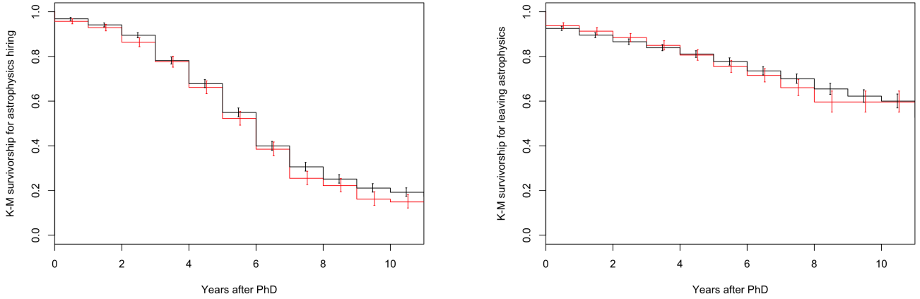
Figure 3. Kaplan-Meier survivorship curves for astronomy PhDs (effectively, the cumulative distribution function corrected for incompleteness and alternative outcomes). The left version shows the hiring time into astronomy careers; the right considers leaving the field (hiring into other careers).
