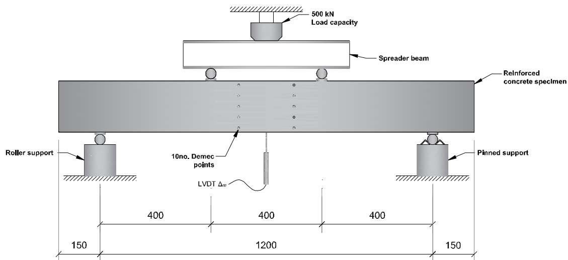
Fig. 4. Schematic test arrangements.
