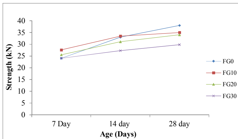
Fig. 2. Development of compressive strength over time
