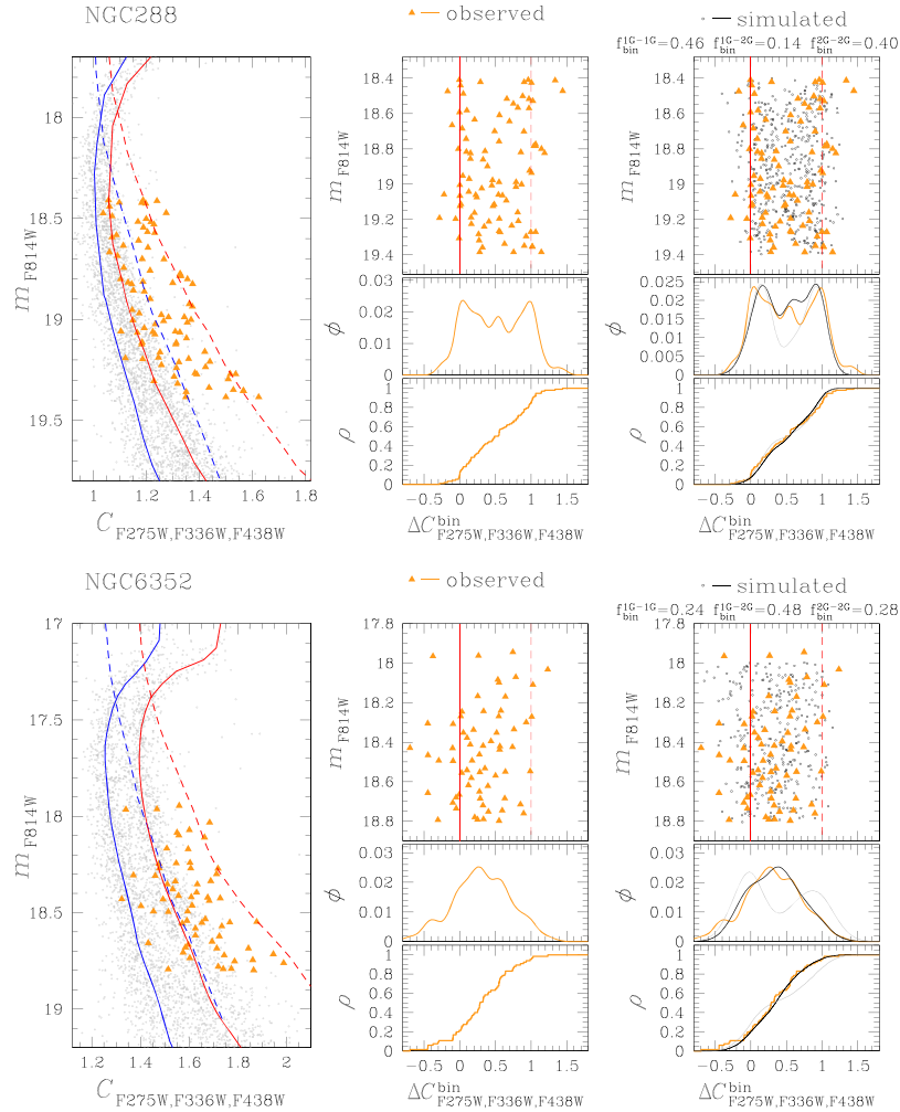
Figure 7 m_{F814W} versus C_{F275W, F336W, F438W} diagrams zoomed-in the upper MS (left). Verticalized m_{F814W} versus \Delta C_{F275W, F336W, F438W}^{bin} for the selected binaries and corresponding kernel-density distribution (middle and right-hand panels). Red and blue continuous lines are the fiducials of 1G and 2G stars, respectively, while the dashed lines with the same colour are the corresponding fiducials for equal-mass binaries. Orange triangles mark the selected observed binaries, whose \Delta C_{F275W, F336W, F438W}^{bin} kernel-density distribution and cumulative distribution is represented with orange lines. Black dots and black lines refer to the simulated binaries. The grey lines correspond to the distributions of \Delta C_{F275W, F336W, F438W}^{bin} for the simulations with no mixed binaries that provides the best match with the data. The fraction of 1G–1G, 1G–2G, and 2G–2G simulated binaries are quoted in the right-hand panels.
