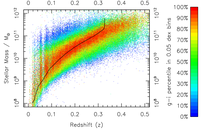
Figure 1. The variable stellar mass redshift selection limit. In each vertical M \pm 0.025 dex bin the cumulative density function (CDF) of apparent g-i colour is calculated. Depending on where a galaxy appears in the CDF given its stellar mass the colour of the data point is different: relatively bluer (redder) g-i colour galaxies are bluer (redder) data points. The black line shows the selection limit and is imposed at the 95 th percentile for each bin.
