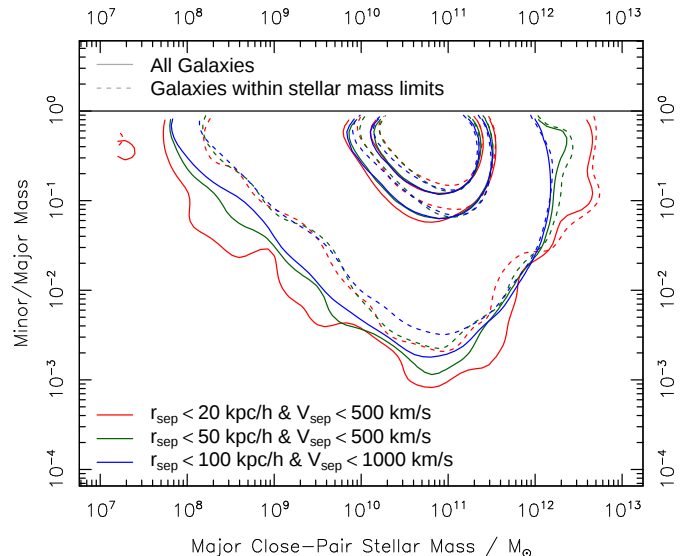
Figure 3. 2D density contours showing the highest density regions containing 50% (inner contours), 68% (middle) and 99% (outer) of the data when comparing the major close-pair stellar mass (x-axis) to the minor/major stellar mass ratio (y-axis). The line definitions are as per Figure 2.
