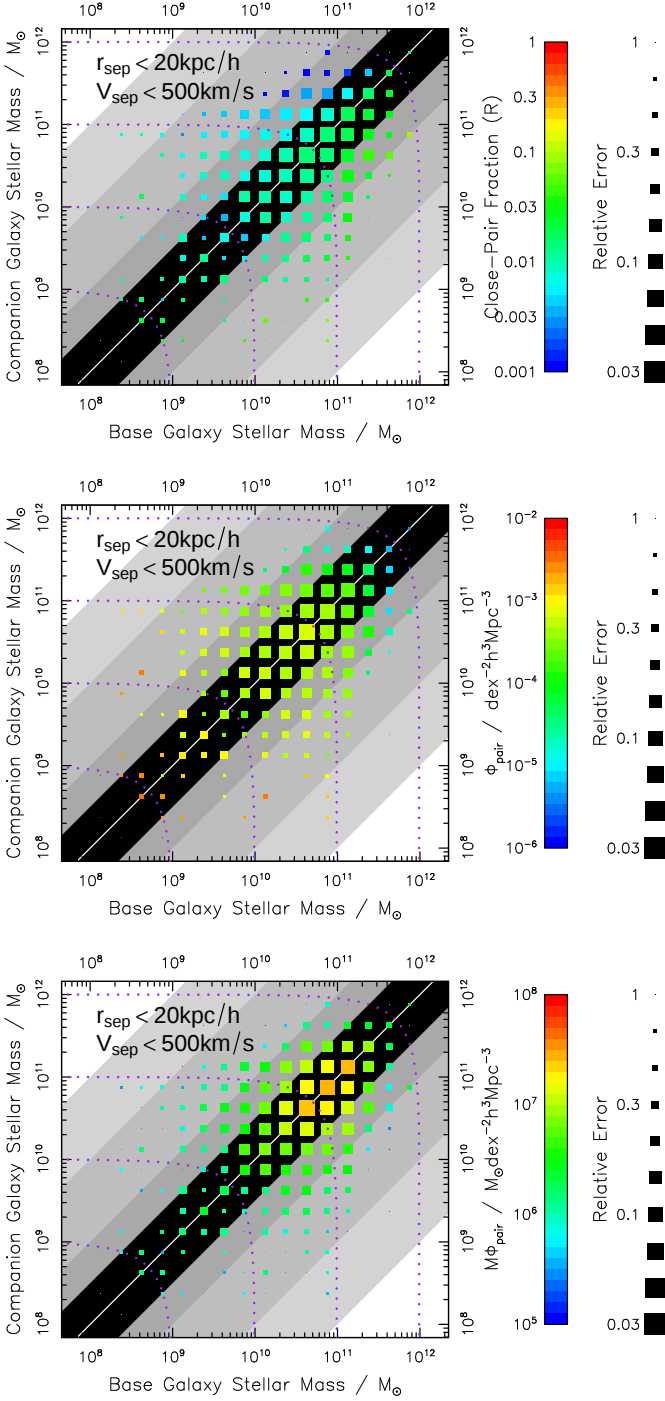
Figure 7. Pair properties for r_{\text{sep}} < 20 \text{ kpc} and v_{\text{sep}} < 500 \text{ km s}^{-1} sample ( PS_{r20v500} ) true pair corrected using the mock catalogues ( W_{TP}\text{-mock} , see Section 3.4). Top panel shows the observed pair fraction for the y-axis companion galaxy per stellar mass interval of the x-axis base galaxy. Middle panel shows the observed pair number density for the y-axis companion galaxy per stellar mass interval of the x-axis base galaxy. Bottom panel shows the observed minor accreting mass stellar mass density for the y-axis pair galaxy per stellar mass interval of the x-axis base galaxy (the number density of the pairs multiplied by the mass of the less massive galaxy in any close-pair). In all panels the black background region shows the regime of major mergers (mass ratio within a factor 0.5 dex), subsequent lightening grey regions show increasing decades in merger mass ratio. The purple lines show different merger mass products ranging from 10^8 M_{\odot} – 10^{12} M_{\odot} .
