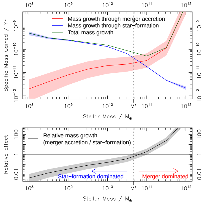
Figure 17. Top panel shows the fraction of mass added to current galaxy stellar mass via various mechanisms. The red line shows the fraction of increase expected via minor galaxy accretion onto galaxies where we use close-pair fractions derived from our most dynamically compact PS_{r20v500} close-pair sample, true pair corrected using the mock catalogues ( W_{TP-mock} , see Section 3.4). The timescale is assumed to be 1 Gyr with a lower limit of 0.5 Gyr and upper limit 2 Gyr, where the red shaded region folds this uncertainty in with the errors in our parameterisation. The blue line shows the effect of taking the Bauer et al. (2013) sSFR at low redshift. The green line is the sum of the red and blue lines (merger accretion and star-formation). The bottom panel shows the mass increase through merger accretion relative to that from star-formation.
