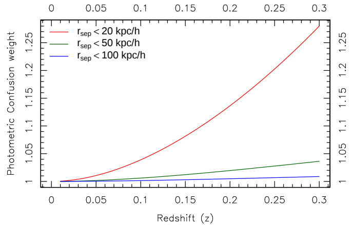
Figure 5. The weighting applied to an observed pair at a given redshift within specified projected separation limits. This accounts for the sharp fall in close-pairs within 3'' on the sky, which at a redshift of 0.3 can be a substantial fraction of the pair search radius.
