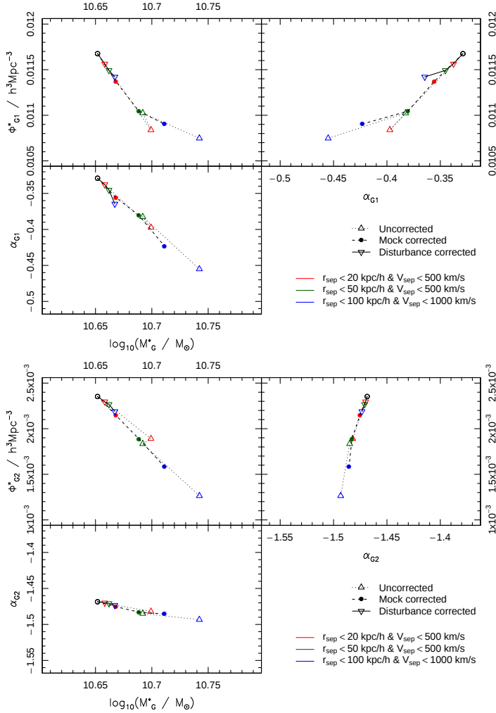
Figure 19. The two sets of panels show the various two-parameter shifts for the Bayesian expectation of the GSMF posterior parameterisation, given different future merger history scenarios. In all panels the original parameter fit is shown by the open black circle.
