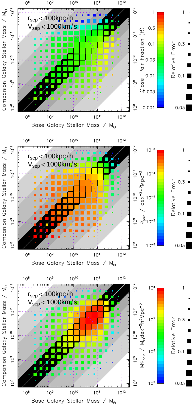
Figure 9. Pair properties for r_{\text{sep}} < 100 \text{ kpc} and v_{\text{sep}} < 1000 \text{ km s}^{-1} sample ( PS_{r100v1000} ) true pair corrected using the mock catalogues ( W_{TP-\text{mock}} , see Section 3.4). For more information see the caption for Figure 7.
