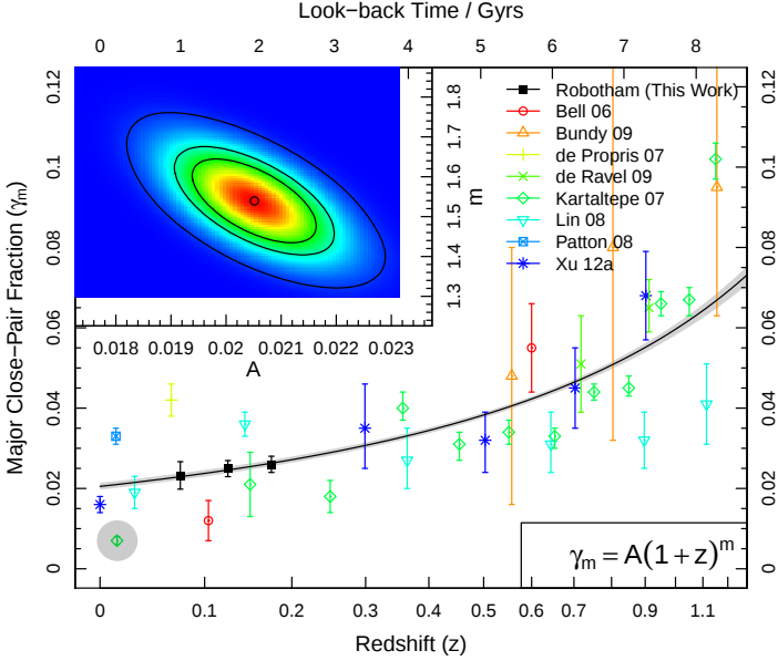
Figure 15. Major merger close-pair fraction as a function of redshift (bottom) or look-back time (top). The stellar mass range explored is limited to z < 0.2 in GAMA since we are still conservatively complete to \mathcal{M}^* galaxies out to this redshift. This Figure uses data taken from Bell et al. (2006); Bundy et al. (2009); de Propriis et al. (2007); de Ravel et al. (2009); Kartaltepe et al. (2007); Lin et al. (2008); Patton et al. (2008); Xu et al. (2012a) as presented in Xu et al. (2012a), where results are scaled so as to use a common 20 h^{-1} kpc projected separation, 500km/s velocity separation and major merger definition of a 3:1 mass ratio close to \mathcal{M}^* . The solid black line shows the Bayesian expectation for our simple 2 parameter model, and the grey shaded region shows the 1\text{-}\sigma marginalized range of allowed fits. The top-left inset panel shows the 50%, 1\sigma and 95% percentile range contours for our preferred model using the posterior MCMC chains.
