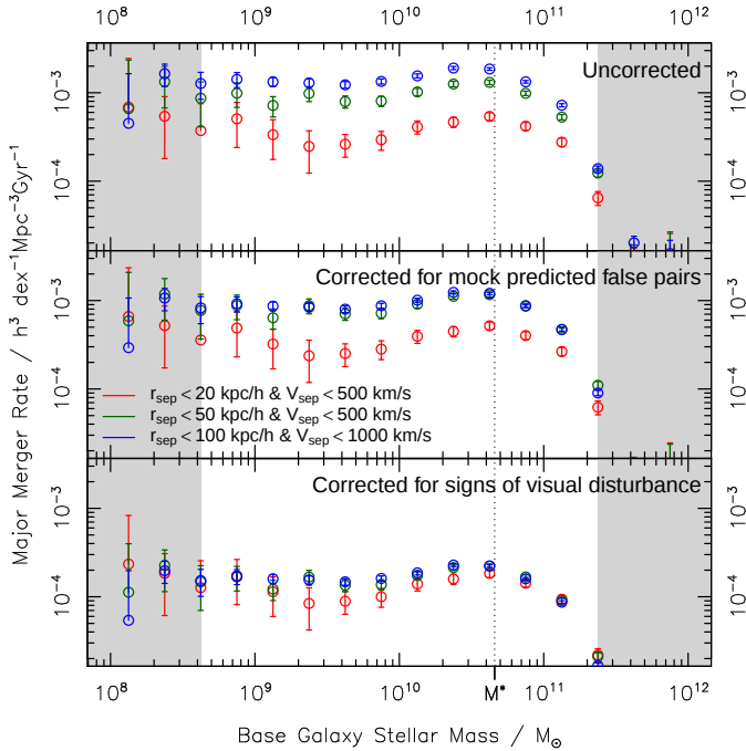
Figure 14. Major merger rates as a function of stellar mass for different dynamical pair selections. This is a simplified representation of the information presented in Figures 7, 8 and 9 combined with estimates of merger timescale for different stellar mass close-pairs taken from Kitzbichler & White (2008). The Kitzbichler & White (2008) mappings naturally account for false close-pairs due to their calibration to simulated data, so we expect the top-panel (applying it to our ‘uncorrected close-pair fractions’) to be the most representative of the true merger rates.
