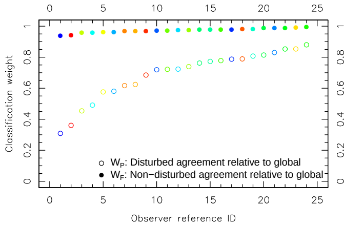
Figure A2. Comparison of classification weights for individual classifiers (24 in total). The classifiers are ordered by their W_F weight, i.e. how consistently their ‘undisturbed’ classification agrees with that of their fellow classifiers. The y-axis indicates the weight used to re-define classification assessments. If a classifier tends to generously flag galaxies as disturbed compared to the global typical classification (left hand side) their weight for such an assessment is decreased. This is not to say the global choice is always better , but for this analysis we want all classifications to be biased in the same way.
