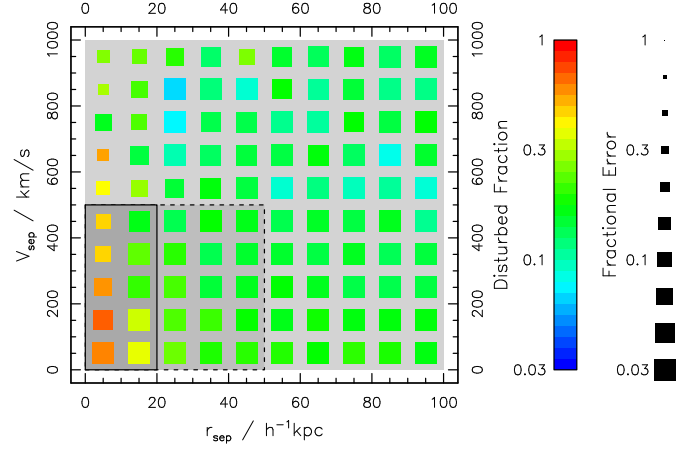
Figure 6. Fraction of galaxies in each dynamical bin showing signs of disturbance. This is corrected for the simplest stellar mass dependent redshift bias (see Figure 4). The darkest grey box with solid lines shows the PS_{r20v500} sample, the next darkest box with dashed lines shows the PS_{r50v500} sample, and the entire plotting region shows the PS_{r100v1000} sample. The size of the box indicates the error, where smaller means less significant, i.e. more error in the measurement.
