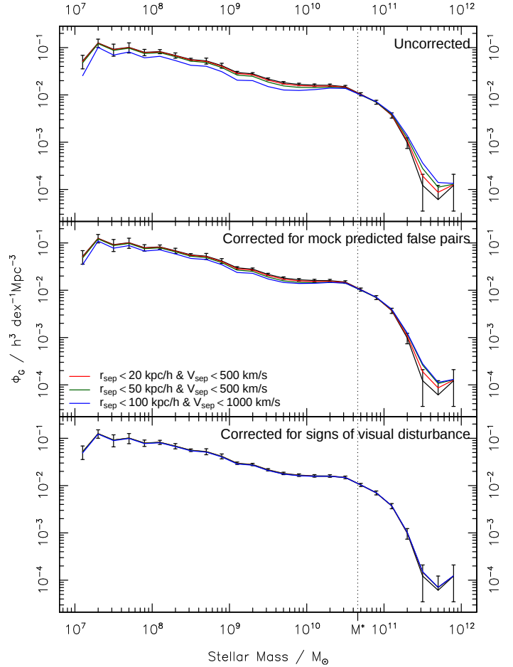
Figure 18. Depiction of the effect on the GSMF presented in Baldry et al. (2012) if the different close-pair selections shown in Figure 16 were assumed to merge on some unknown timescale. The top panel is only corrected for galaxies appearing in multiple close-pairs. The middle panel is true pair corrected from the mock catalogues using W_{TP-mock} (see Section 3.4). The bottom panel is corrected for the fraction of visually disturbed galaxies in pairs using W_{TP-vc} (see Section 3.4). In all cases mass is moved from moderate stellar mass galaxies ( 10^8 M_\odot – 10^{10} M_\odot ) to beyond \mathcal{M}^* (although this is hard to identify in the bottom panel). This has the inevitable effect of enhancing the dip in this regime, increasing the significance of the double-Schechter shape in the GSMF and moving the future value of the GSMF \mathcal{M}^* to larger masses.
