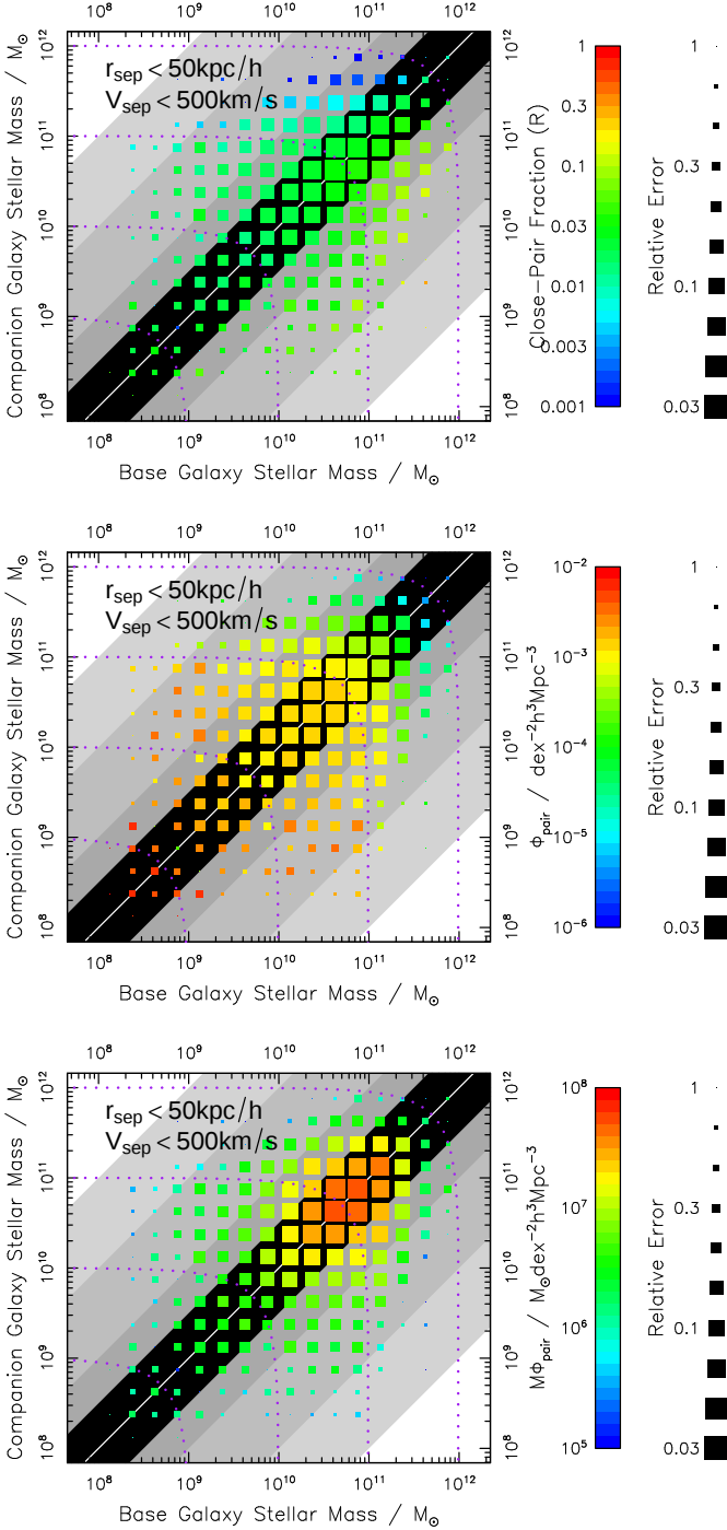
Figure 8. Pair properties for r_{\text{sep}} < 50 \text{ kpc} and v_{\text{sep}} < 500 \text{ km s}^{-1} sample ( PS_{r20v500} ) true pair corrected using the mock catalogues ( W_{TP-mock} , see Section 3.4). For more information see the caption for Figure 7.
