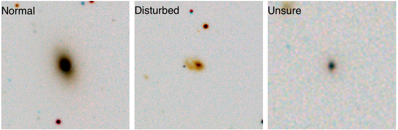
Figure A1. The three classifications of galaxy disturbance used in this work. All images used are 60 h^{-1} \text{ kpc} \times 60 h^{-1} \text{ kpc} in physical distance and linearly map g/r/K SDSS and VIKING flux data onto blue, green and red colours which are then inverted. This means visually redder colours correspond to bluer g-r colours in the original images. The left panel is an example of a ‘normal’ galaxy that does not show signs of morphological disturbance, the middle panel is an example of a ‘disturbed’ galaxy and the right panel is an example of a galaxy where our classification would be ‘unsure’ because there are so few pixels of information. Images were randomly selected from the close-pairs subset (i.e. all of them have known close-pair companion galaxies, and none are taken from the isolated control sample).
