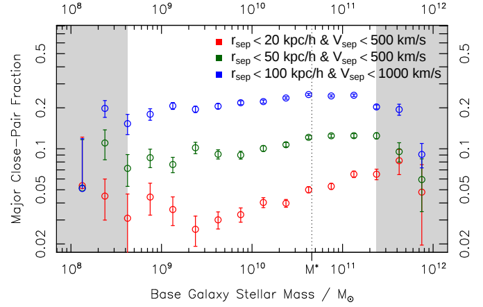
Figure 13. Major merger fractions as a function of stellar mass for different dynamical pair selections. This is a simplified representation of the information presented in Figures 7, 8 and 9.
