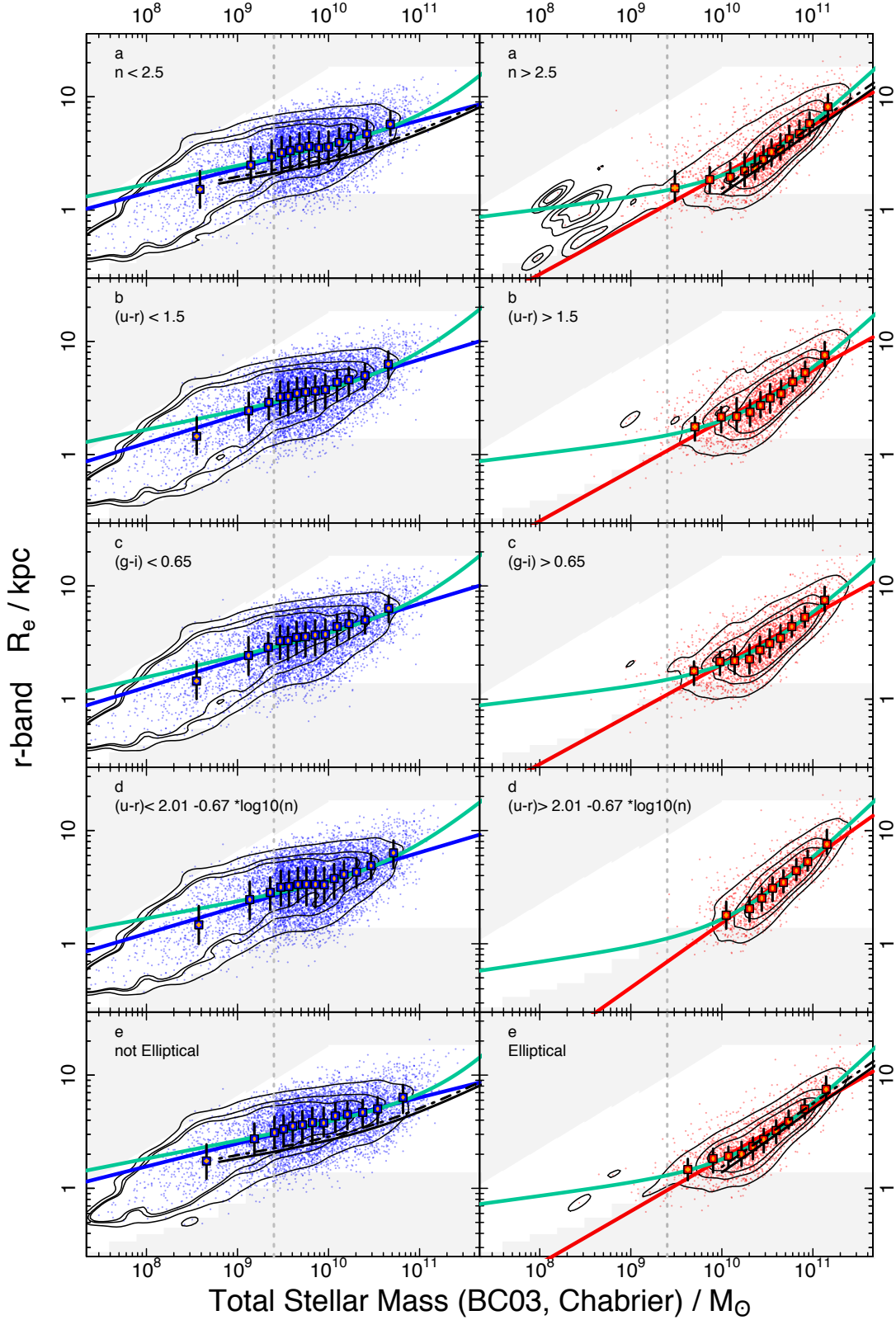
Figure 3. The \mathcal{M}_* - R_e relation for early- (red, right hand side) and late- (blue, left hand side) type galaxies divided by: a) Sérsic index n ; b) Dust corrected colour (u-r)_{stars} ; c) Dust corrected colour (g-i)_{stars} ; d) Rolling Sérsic index division and e) Visual Elliptical/Not-Elliptical classification. The red and blue lines are single power-law fits to the binned data (Eq. 2), the green lines are two component power-law fits (Eq. 3) and the grey dotted line indicates the lower mass limit highlighting the wealth of data that have been ignored. The grey shaded areas indicate where measurements become less reliable due to our detection limitations. The black solid and dot-dashed lines in panels a) and e) show the S03 \mathcal{M}_* - R_e relation where the dot-dashed line shows the sizes corrected from z- to r-band values and the solid line shows the relation as is. For the fitting parameters see Tables 2 and 3.
