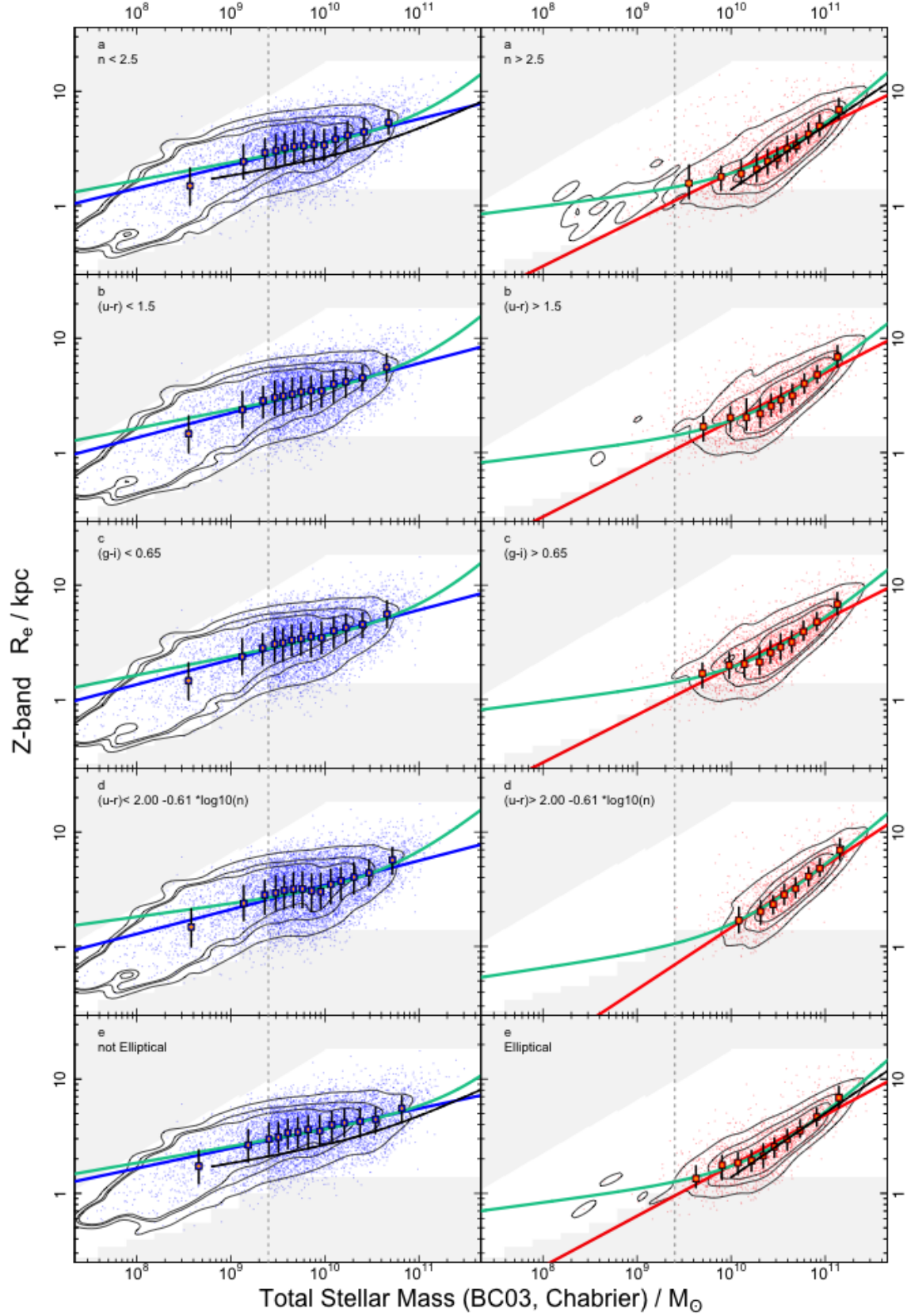
Figure A5. The \mathcal{M}_* - R_e relation for the VIKING Z-band with the panels and fits as in Fig. A1.
