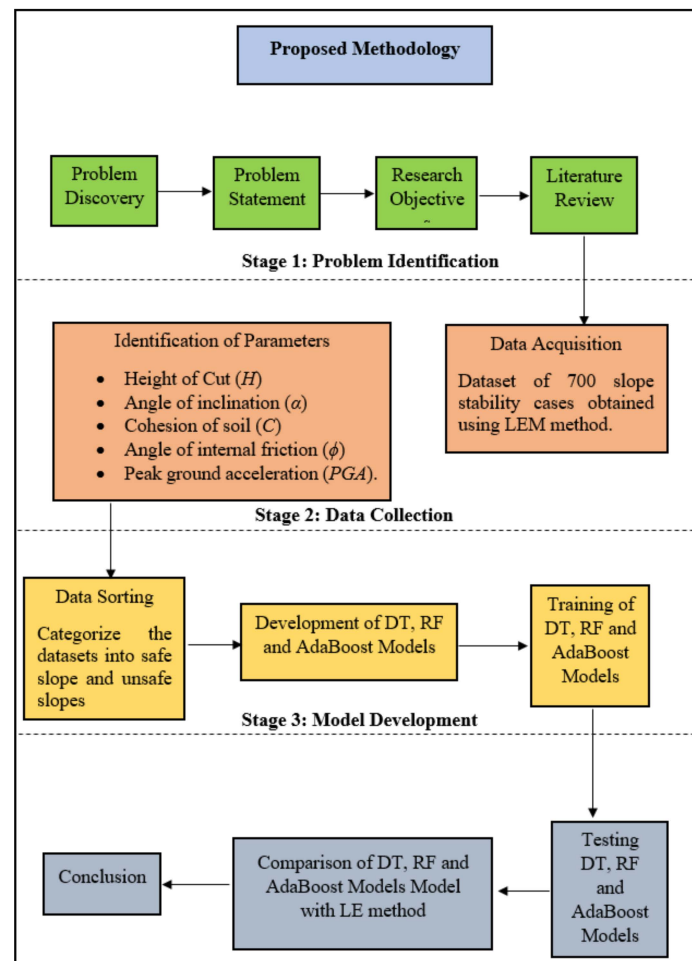
Figure 2. Procedure flowchart for FOS classification.
