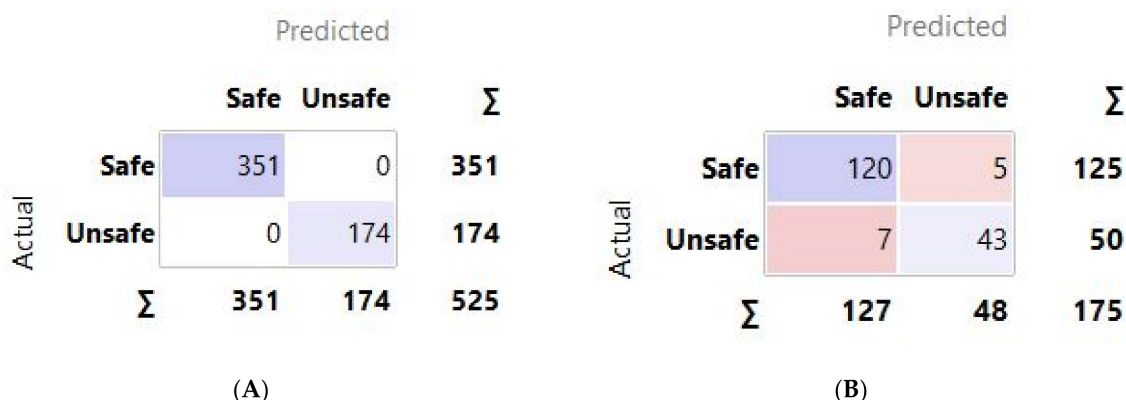
Figure 9. The AdaBoost model results for FOS classification: (A) Training and (B) Testing.
