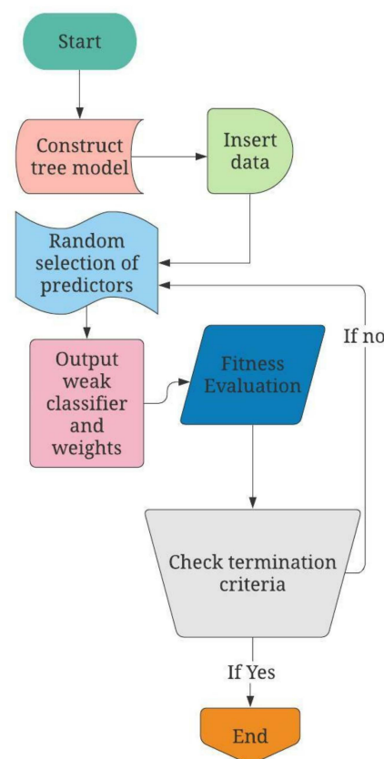
Figure 5. Methodology flowchart for AdaBoost modelling.
