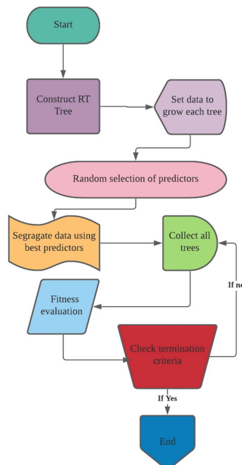
Figure 4. Methodology flowchart for RF modelling.
