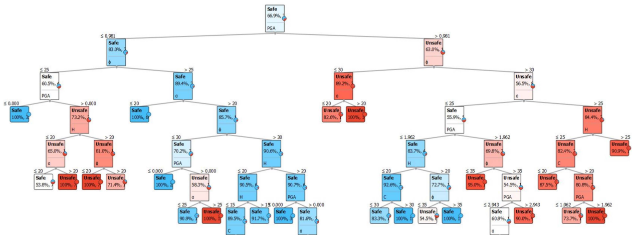
Figure 6. The optimal DT model for FOS classification.
