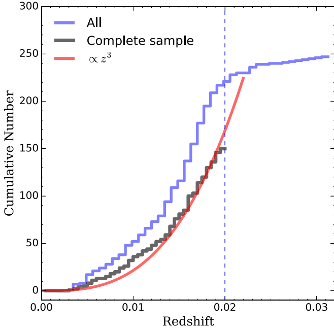
Figure 1. The cumulative redshift distribution of all SNe Ia (blue histogram) in DR1 and those in the complete sample (black histogram) from the CN1a0.02 project. The redshift limit of z = 0.02 for the complete sample is indicated with the dashed vertical blue line. An illustrative N \propto z^3 is plotted with the red line to indicate a simplified expectation from a volume-limited sample covering the full luminosity range by assuming a linear relation between distance and redshift. The distribution approximately follows the expectation for a volume-limited sample at z \gtrsim 0.01 , for which peculiar velocities are negligible compared to the Hubble expansion velocity. The apparent excess of SNe with 0.005 \lesssim z \lesssim 0.013 with respect to the volume-limited expectation is probably contributed by the effects of peculiar velocities at low redshift and/or fluctuations due to small number statistics.
