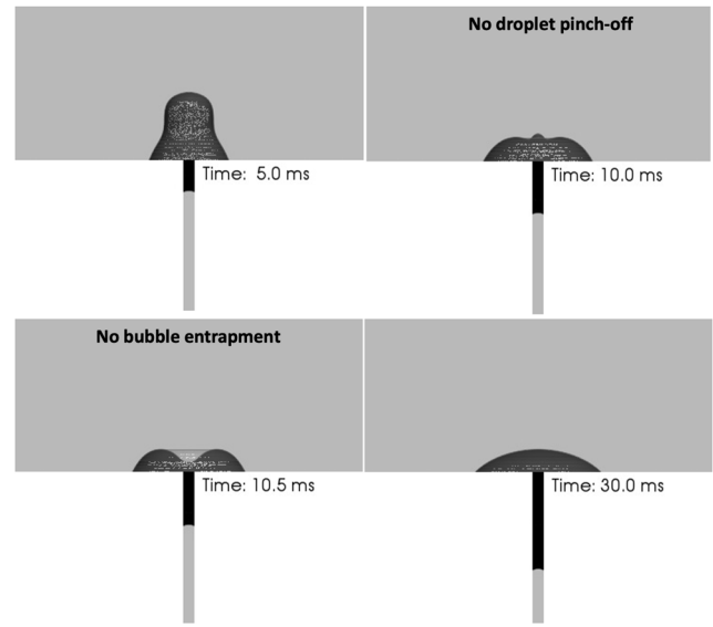
FIG. 16. Indicative droplet evolution for the case with a pore radius of r_{\text{pore}} = 0.2 \text{ mm} and a liquid kinematic viscosity of \nu = 8 \times 10^{-6} \text{ m}^2/\text{s} (case 3-8 from Table I).
