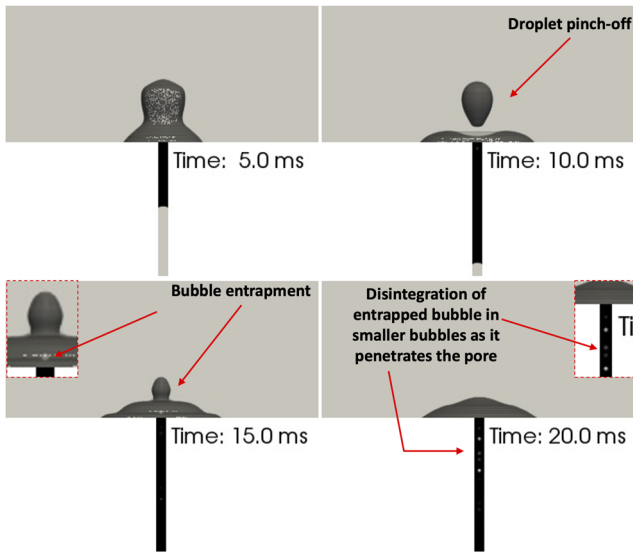
FIG. 15. Indicative droplet evolution for the case with a pore radius of r_{\text{pore}} = 0.2 \text{ mm} and a liquid kinematic viscosity of \nu = 1 \times 10^{-6} \text{ m}^2/\text{s} (case 3-1 from Table I).
