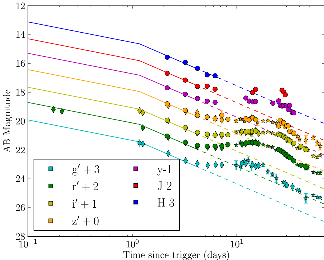
FIG. 1.— Optical and NIR light curves of GRB 130702A, corrected for Galactic extinction and host extinction (assuming A_{V,\text{host}} = 0.10 ). Note that the host galaxy contribution is not removed. Diamonds are P48/P60 data, circles are RATIR data, and stars are Liverpool data; errorbars are overlotted on all datapoints. Solid lines indicate power-law fits with \alpha_1 = 0.57 and t_b = 1.17 d taken from Singer et al. (2013a) and \alpha_2 = 1.25 from the XRT power law decay index. Dashed lines mark the extrapolated power law where we assume \alpha_2 for all times beyond t_b .
