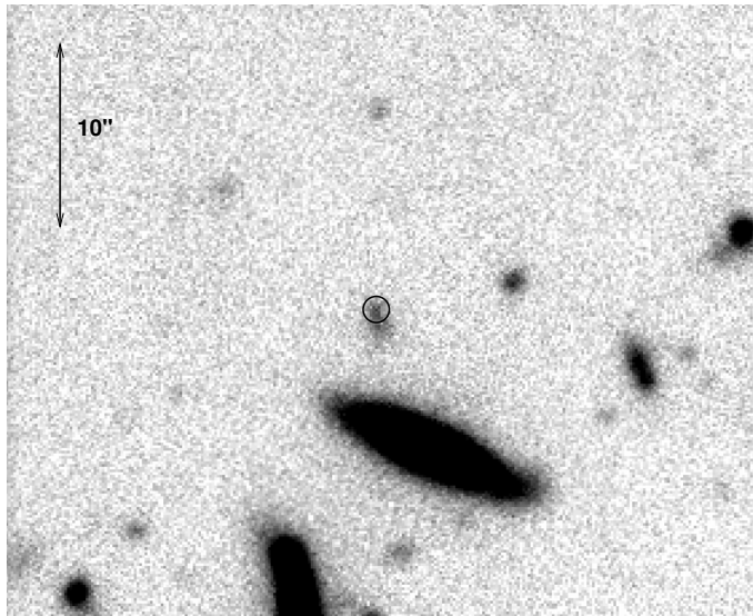
FIG. 2.— Keck/LRIS g' -band image of the host galaxy of GRB 130702A, obtained at \Delta t = 330.48 d after the GBM trigger (i.e., when the afterglow and SN emission had faded away). The location of the transient is indicated by the black circle ( 0''.5 radius, significantly larger than the actual astrometric uncertainty). The dwarf host is clearly elongated in the N-S direction, with the bulk of the star formation (as evidenced by the transient location and the nebular emission lines) apparent in the northern component. The image is oriented with N up and E to the left.
