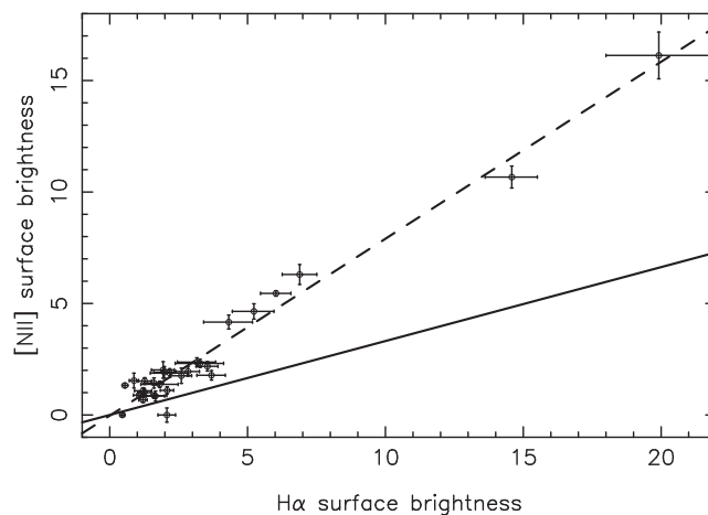
Figure 9. [NII] surface brightness versus H\alpha surface brightness within SFD regions, both measured in units of 10^{-20} \text{W m}^{-2} \text{arcsec}^{-2} . H\alpha emission has been corrected for underlying absorption by a 3–4 Gyr old stellar population. The solid line corresponds to the mean emission-line ratio ( [NII]/H\alpha = 0.332 ) found for HII regions in the same galaxy sample.
