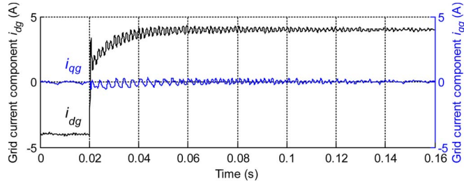
Fig. 20. Grid current components i_{dg} and i_{qg} , during transition from V2G to charging mode, obtained within the controller after grid current transformation into voltage-oriented reference frame.
