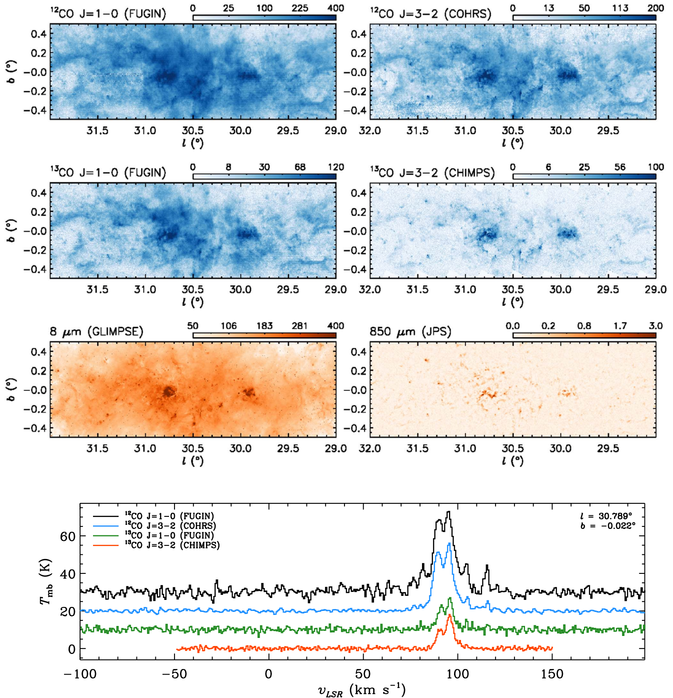
Figure 8. W43 star-forming region within the COHRS coverage area. From the top left to the bottom, each panel displays ^{12}\text{CO} (1–0) FUGIN data, ^{12}\text{CO} (3–2) COHRS data, ^{13}\text{CO} (1–0) FUGIN data, ^{13}\text{CO} (3–2) CHIMPS data, 8\ \mu\text{m} GLIMPSE data, 850\ \mu\text{m} JPS data, and examples of CO spectra, respectively. The CO maps are velocity-integrated over the v_{\text{LSR}} range of (80, 110)\ \text{km s}^{-1} (Nguyen Luong et al. 2011), and the units on the intensity scale of the integrated main-beam temperature are \text{K km s}^{-1} . The units on the intensity scale of the GLIMPSE and JPS data are \text{MJy sr}^{-1} and \text{Jy beam}^{-1} , respectively. The CO spectra were obtained at the position closest to the velocity-integrated ^{12}\text{CO} (3–2) emission peak. The offsets of 10 K, 20 K, and 30 K to the spectra have been added for better visualization.
