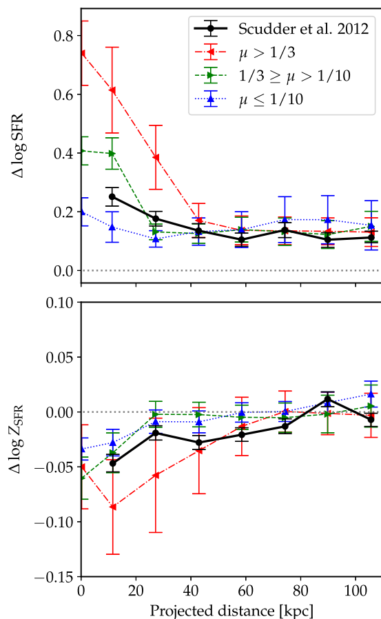
Figure 4. Fractional change of the SFR (top panel) and the metallicity (bottom panel) as a function of projected distance for our sample of galaxies (dashed lines) and the observations of Scudder et al. 2012 (solid lines). The error bars show the standard error of the median. The observed sample shows SFR-enhancement at r < 40 kpc and metallicity dilution at r < 60 kpc. For our simulated sample, major mergers show SFR-enhancement at r < 30 kpc and dilution at r < 40 kpc. For minor mergers, SFR-enhancement and dilution occur at the same distances, within r < 30 kpc. The fractional changes are progressively stronger for larger mass ratios and smaller distances, with the exception of major mergers, where the dilution peak occurs at a distance \sim 10 kpc, which is slightly increasing with the coalescence time. This is caused by stellar metal enrichment overcoming the dilution.
