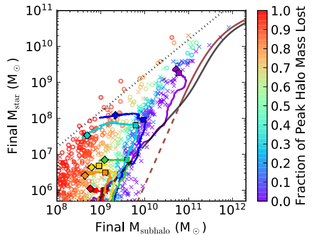
Figure 10. The final stellar mass versus final halo mass for all resolved systems within 1Mpc of the host galaxies in all 30 Auriga simulations. Open circles are systems within R_{200} at z = 0 and xs are systems beyond R_{200} . The colour of these points indicate the fraction of their total halo mass that has been lost from their peak mass as measured from their merger trees: red points have lost over 90 per cent of their halo mass and purple points have lost very little mass. Coloured lines show the evolutionary tracks of a few example systems from Au6 in this plane. Along these tracks, squares indicate the point at which the system first crosses within R_{200} and diamonds indicate their final position. The black dotted line indicates the cosmic baryon fraction \Omega_b/\Omega_m . The brown solid/ dashed line indicates an abundance matching estimate for central dark matter haloes taken from Guo et al. (2010) and the black solid/dashed line indicates an estimate from Behroozi, Wechsler & Conroy (2013). For both these trends, the solid portion of the line covers the portion of parameter space where these studies make predictions and the dashed lines are power-law extensions of the estimated trends to lower masses.
