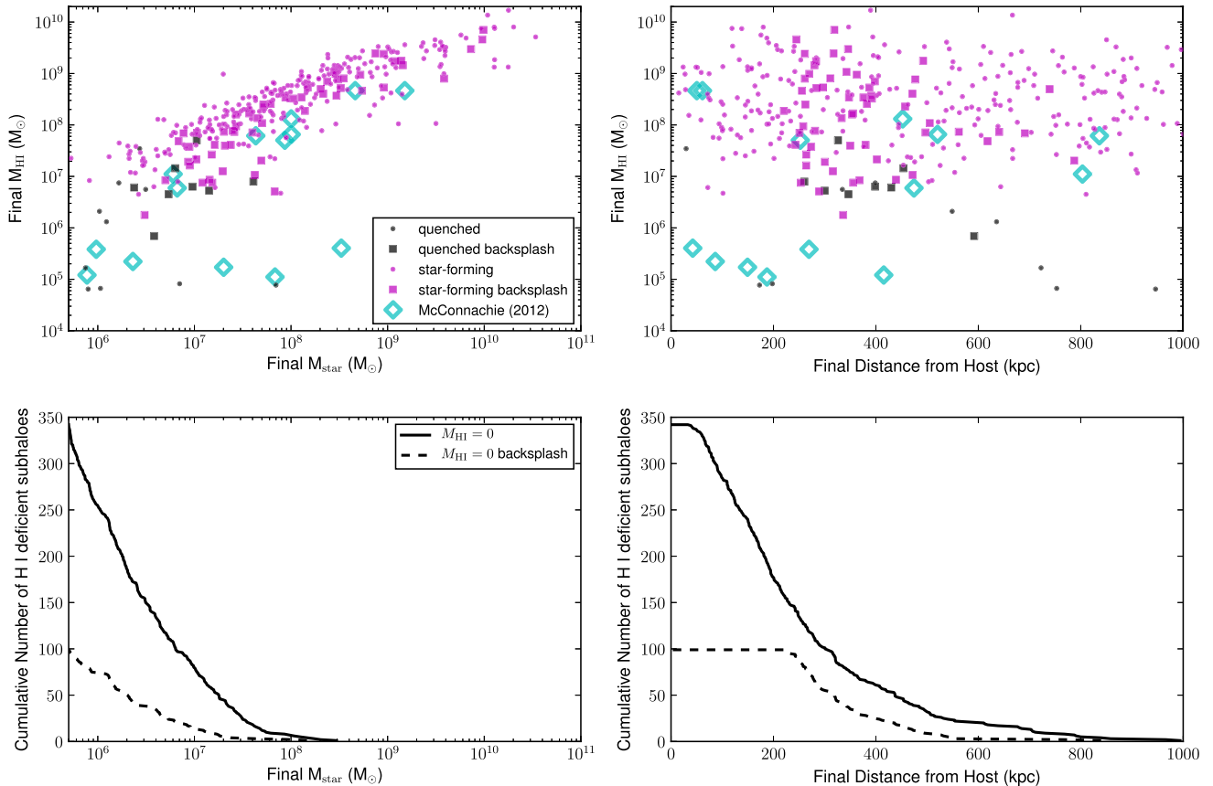
Figure 3. H\text{I} masses of subhaloes within 1 Mpc versus final stellar mass (top left) and final distance from the host (top right). All systems with non-zero H\text{I} masses are shown. Quenched systems are shown with black points and star-forming systems are shown with magenta points. ‘Backslash’ systems (systems beyond R_{200} at z = 0 that have passed within R_{200} at some earlier redshift) are shown with squares; satellites and non-backslash isolated systems are shown with circles. Measured H\text{I} masses of Local Group systems within 1 Mpc of either the MW or M31 (McConnachie 2012) are also shown (cyan diamonds). Systems that have zero H\text{I} masses are shown in the lower panels: cumulative distributions of the number of H\text{I} deficient systems with stellar masses greater than plotted value (left) and the number of H\text{I} deficient systems with final distances greater than the plotted value (right). Distributions for H\text{I} deficient backslash systems are shown with dashed lines. Most H\text{I} systems have lower stellar masses and/or are closer to their host.
