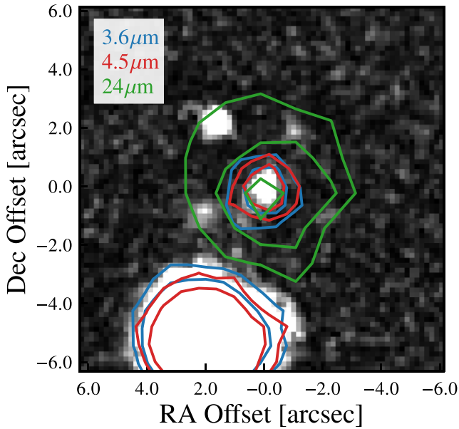
Figure 5. Figure showing the Spitzer /IRAC 3.6 \mu\text{m} (blue), 4.5 \mu\text{m} (red), as well as Spitzer /MIPS 24 \mu\text{m} (green) emission around COS-87259. We show 7\sigma and 12\sigma contours for IRAC, and 4\sigma , 6\sigma , and 8\sigma contours for MIPS. The background image is the near-IR stack centred on the rest-UV position of COS-87259. The centroids of each Spitzer detection near COS-87259 are closely aligned with the rest-UV centroid ( <0.5 arcsec) and there is no evidence of significant confusion impacting any of the Spitzer detections.
