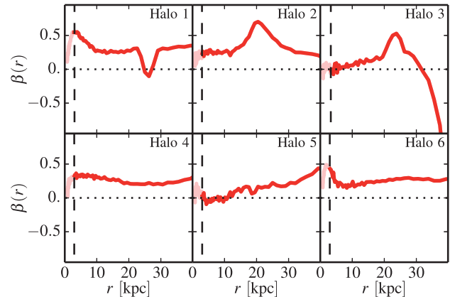
Figure 8. Stellar anisotropy profile \beta(r) as a function of radius for the six EAGLE clusters over the radial range relevant to the stellar kinematics analysis. The vertical dashed line on each panel shows the 3D convergence radius, r_c and the profiles at lower radii are shown using shaded lines. Two BCGs are consistent with \beta = 0 but would be better fit with a non-constant \beta . Ignoring complex features, the other four clusters present more radially biased orbits with \beta(r) \approx 0.25 . A single profile shape for \beta(r) cannot be used to characterize all six of our BCGs.
