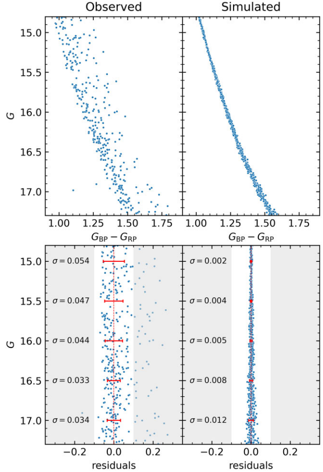
Figure 4. Top panels: Observed (left) and simulated (right) CMDs of the lower MS of M38. Bottom panels: Colour residuals as a function of the G magnitude around the observed (left) and the synthetic (right) CMD fiducials. The area shown in white contains the stars employed to compute the 1\sigma values of the dispersion of the residuals also shown in the two panels (see text for details).
