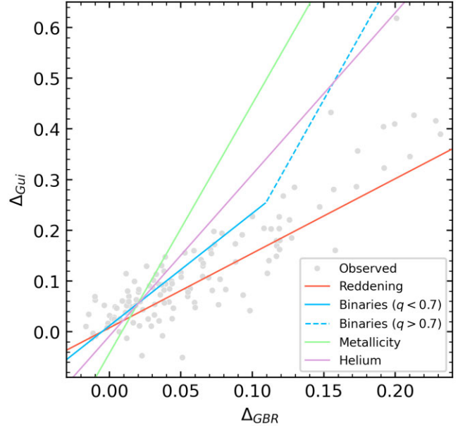
Figure 8. \Delta_{GBR}-\Delta_{Gui} diagram for the lower MS stars. The lines show the directions along which stars would be displaced by differential reddening, unresolved binaries, and initial chemical spread (see text for details).
