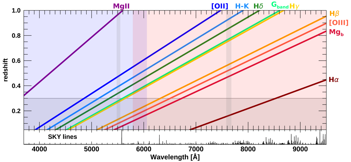
Fig. 2. Observability of the main spectral indices as a function of redshift ( 0.05 < z < 1.0 ) in the wavelength range covered by the WEAVE spectrograph in its low-resolution mode. The visibility of other emission/absorption lines is easily extrapolated from adjacent indices. The blue (red) region indicates the wavelength range covered by the blue (red) arm of the WEAVE spectrograph, and the overlap region covered by both arms is shaded in violet. The two narrower vertical grey bands are CCD gaps in the blue and red arm of the WEAVE spectrograph. They indicate the redshift ranges in which some of the features will not be available in observations. The empty region shows the redshift range in which the large majority of StePS targets will be observed ( z \geq 0.3 ). The bottom panel shows an OH sky lines spectrum for reference.
