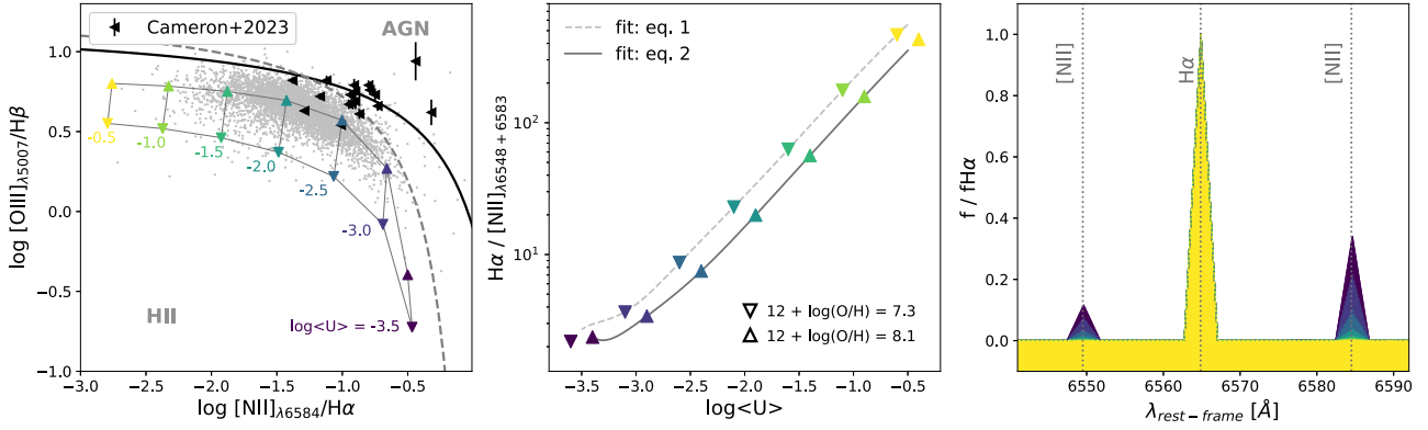
Figure 2. Summary of the Cloudy models used in this work, showing the relative intensity of [\text{N II}] in comparison to \text{H}\alpha . As the ionization parameter ( \log \langle U \rangle ) increases, the [\text{N II}] emission decreases. Specifically, for the parameter space populated by high redshift galaxies ( \log \langle U \rangle \gtrsim -2.5 ), [\text{N II}] is negligible compared to \text{H}\alpha . The coloured triangles represent two different stellar and gas-phase metallicities, as labelled. Left panel: BPT diagram showing the SDSS sample (grey points) and the evolution of CLOUDY models with varying ionization parameter values. Also shown are the [\text{O III}]/\text{H}\beta measurements and [\text{N II}]/\text{H}\alpha upper limits for galaxies at z \sim 6 from Cameron et al. (2023) (black sideways triangles). Middle panel: evolution of the [\text{N II}]/\text{H}\alpha ratio with increasing \log \langle U \rangle . Right panel: zoom-in of spectral region enclosing \text{H}\alpha and [\text{N II}] , normalized to the \text{H}\alpha peak. The [\text{N II}] emission is colour-coded by \log \langle U \rangle .
