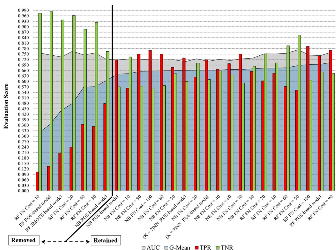
Fig. 11 Filtered models and their associated TNR, TPR, G-Mean and AUC-ROC test performances
