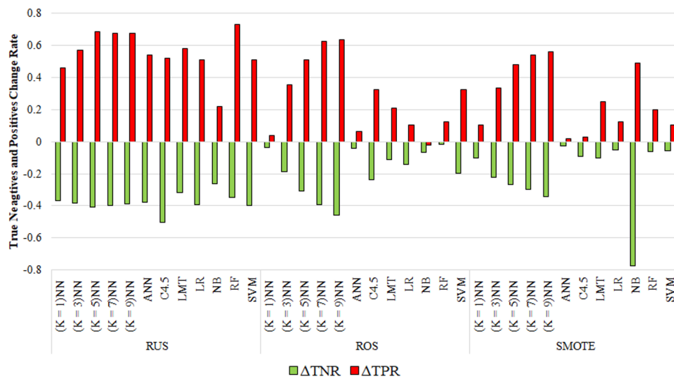
Fig. 8 TN and TP change rates in test per classifier in RUS, ROS and SMOTE models
