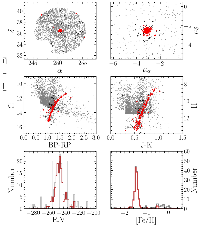
Figure 2. Selecting M13 members in the APOGEE catalogue. In all panels, grey dots represent catalogue stars within 4r_j of the GC centre. Black dots represent stars whose PMs differ from the mean value from the VB catalogue by no more than 4\sigma_{PV} . Red dots represent a subsample of the former whose RVs differ from the GC mean by no more than 3\sigma_{RV} .
