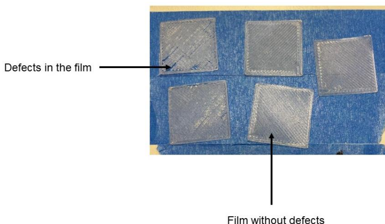
Figure 6: Photographs of 3D printed films.
