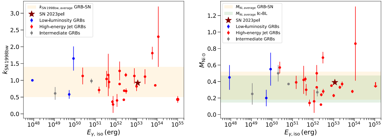
Figure 7. Left panel: modification of Figure 5 from Srinivasaragavan et al. (2023), where k_{\text{SN}1998\text{bw}} is plotted against the isotropic equivalent gamma-ray energy ( E_{\gamma,\text{iso}} ) for observationally confirmed GRB-SNe. The plot distinguishes between low-luminosity GRBs, high-energy jet GRBs, and GRBs in the intermediate regime and also shows the average k_{\text{SN}1998\text{bw}} for GRB-SNe in the plot and its dispersion without accounting for GRB 230812B/SN 2023peI. We indicate the results from this work, GRB 230812B/SN 2023peI, with a maroon star. Right panel: a similar update of Figure 5 from Srinivasaragavan et al. (2023), where the M_{\text{Ni}} in M_{\odot} of GRB-SNe is plotted against the isotropic equivalent gamma-ray energy ( E_{\gamma,\text{iso}} ) from the prompt emission for the GRBs. The same distinctions for GRBs are made as for the left panel, and we show the results from this work with a maroon star. We also show the average M_{\text{Ni}} , along with its dispersion, for GRB-SNe in the plot, with the exception of GRB 230812B/SN 2023peI, as well as GRB 221009A/SN 2022xiw, because only a robust upper limit was derived for the event from Srinivasaragavan et al. (2023). We also show the average M_{\text{Ni}} , along with its dispersion, for the Type Ic-BL SN sample not associated with GRBs from Taddia et al. (2019).
