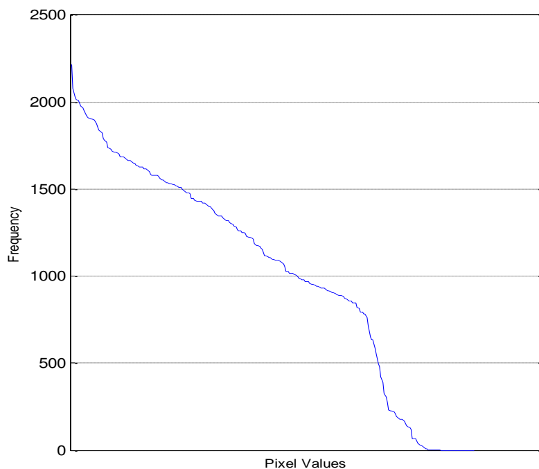
Figure 2: The frequency distribution of the pixel values of the test image Barbara.bmp (512×512) plotted in descending order
