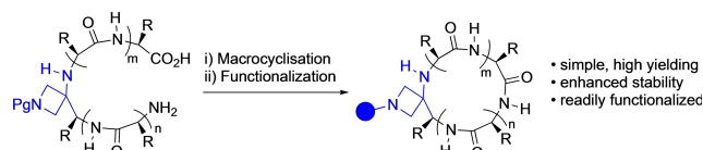
Scheme 1. a) Strategies for the synthesis of small macrocyclic peptides. b) Previous work involving the use of 3-aminooxetanes to improve the macrocyclization of small peptides. c) An overview of this work.
