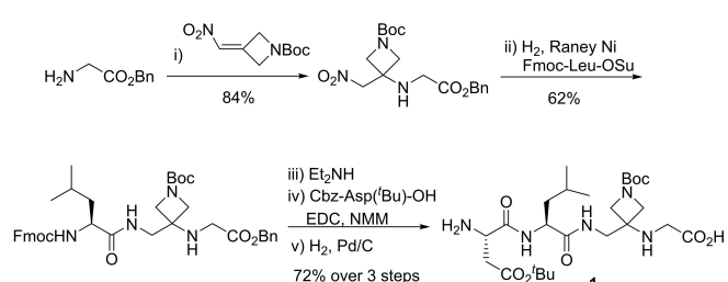
Scheme 1. a) Strategies for the synthesis of small macrocyclic peptides. b) Previous work involving the use of 3-aminooxetanes to improve the macrocyclization of small peptides. c) An overview of this work.
