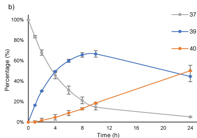
Scheme 6. Analysis of \alpha -chymotrypsin degradation of cyclic peptides. a) HPLC data for cyclo(Thr-Asp-Lys-GAz-Trp-Gly) ( 38 ) over a period of 24 h with GAZ being the azetidino-modified glycine. b) Peptide peak percentage for \alpha -chymotrypsin assay over time for cyclo(Thr-Asp-Lys-Gly-Trp-Gly) ( 37 ) (grey) and linear degradation products H-Gly-Thr-Asp-Lys-Gly-Trp-OH ( 39 ) (blue) and H-Asp-Lys-Gly-Trp-OH ( 40 ) (orange). Peak intensity calculated using analytical HPLC traces. Assay conditions: hexapeptide (200 \mu L, 1.5 mM), \alpha -chymotrypsin (200 \mu L, 50 \mu M), 37 ^{\circ} C, 24 h; final peptide concentration 750 \mu M, \alpha -chymotrypsin concentration (25 \mu M). See ESI, pp62-70† for full assay development.
