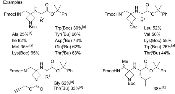
Scheme 2. Strategies for the synthesis of azetidine-modified linear peptides. For full details, see the ESI, pp5–58†. [a] Yield over 2 steps with isolation of the intermediate nitroalkane. [b] Isolated as a 2:1 mixture of diastereomers after column chromatography.
