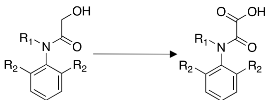
Fig. 3. Metabolic relationships between the category members outlined in Table 3 ( R_1 = alkyl ether or ethyl pyrazole; R_2 = methyl or ethyl).
