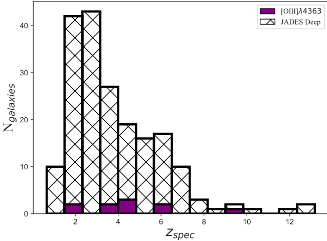
Fig. 1. Redshift distribution of our parent JADES sample of 198 objects with both PRISM and grating spectra and our ten novel [OIII] \lambda 4363 emitters. No pre-selection was performed on the parent JADES sample as we visually inspected all the objects.
