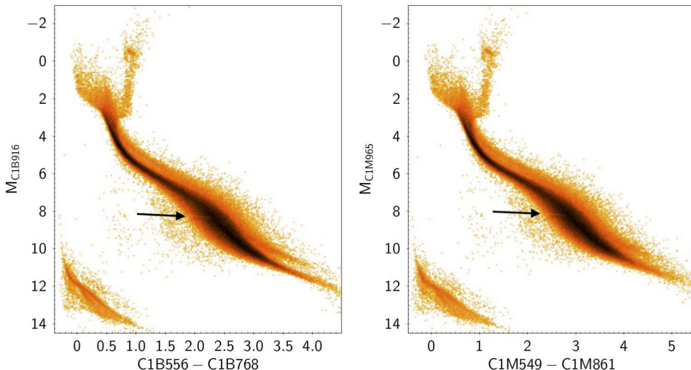
Fig. 23. Two examples of distance-corrected colour magnitude diagrams of the subset of the GCNS catalogue for which XPSP can be obtained, using combinations of broad ( left panel ) and medium width ( right panel ) passbands of the C1 system. Black arrows highlight the location of the Jao gap (Jao et al. 2018), which is clearly visible in both diagrams, showing the high precision of the XPSP in these bands.
