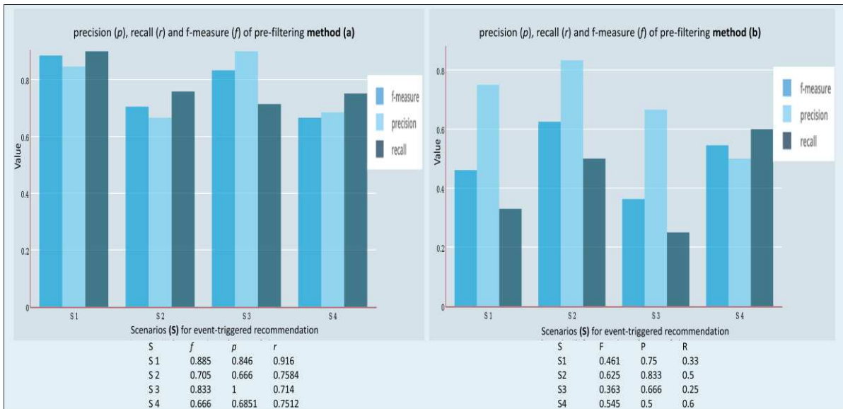
Figure 5. Results for applying pre-filtering methods (a) and (b) on event-based recommendation scenarios 1- 4
