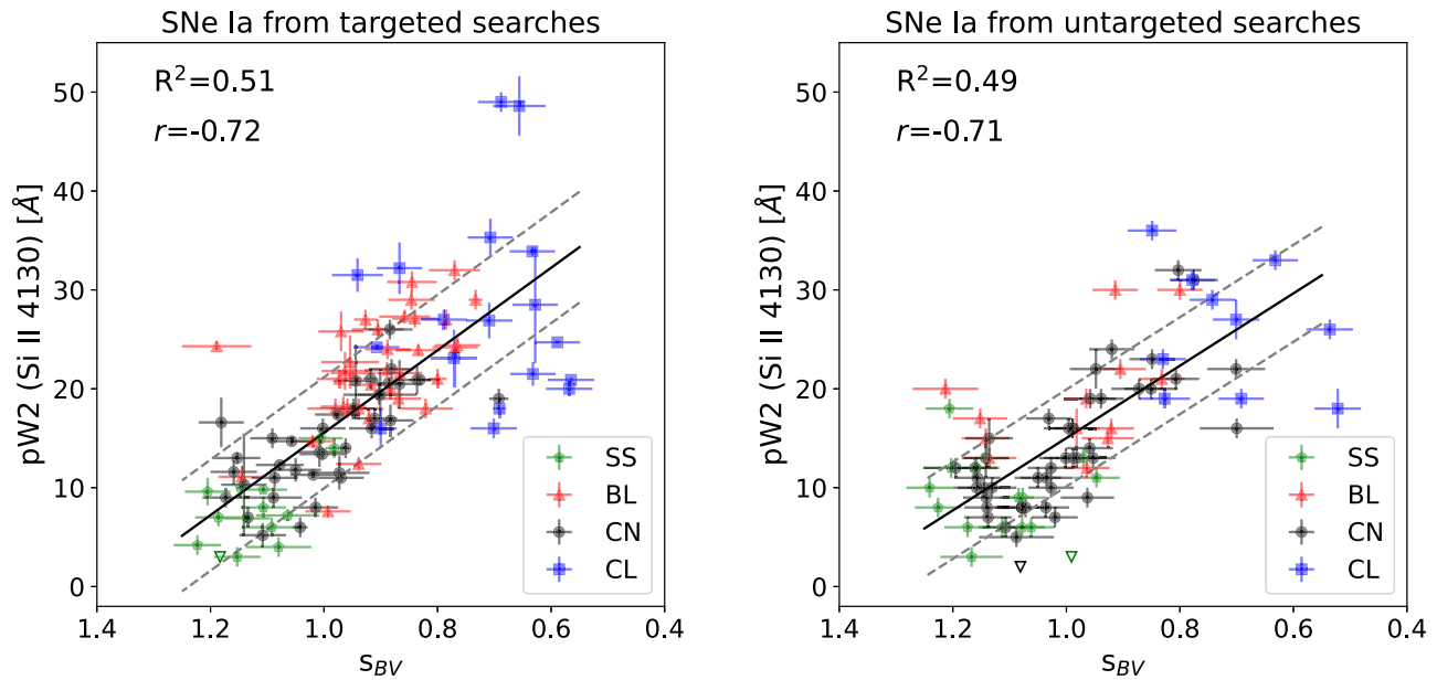
Figure 16. \rho W at maximum light of Si II \lambda 4130 vs. color stretch for our two different samples of SNe Ia discovered by targeted (left) and untargeted (right) searches. The meaning of the symbols is as in Figure 4. The slopes of the best-fit lines are -41.7 \text{ \AA} \pm 4.1 and 36.6 \text{ \AA} \pm 4.0 for the targeted and untargeted samples, respectively. Note that the abscissa ( s_{BV} ) is inverted in this plot to facilitate comparison with Figure 15.
