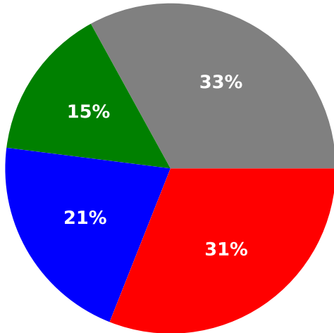
Figure 5. Pie charts showing the incidence of the different Branch types of SNe Ia in our targeted and untargeted samples, respectively.
