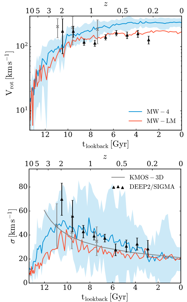
Figure 12. Evolution of the rotation velocity (top panel) and vertical velocity dispersion (bottom panel) of the SF gas for the Milky Way-mass simulations (as shown in Fig. 11). We show observational data points from Simons et al. (2017) for galaxies in the stellar mass range 10^{10} - 10^{11} M_{\odot} , and the binned KMOS-3D data (points and error bars indicate the mean and standard deviation) as well as the best-fitting relation from Übler et al. (2019).
