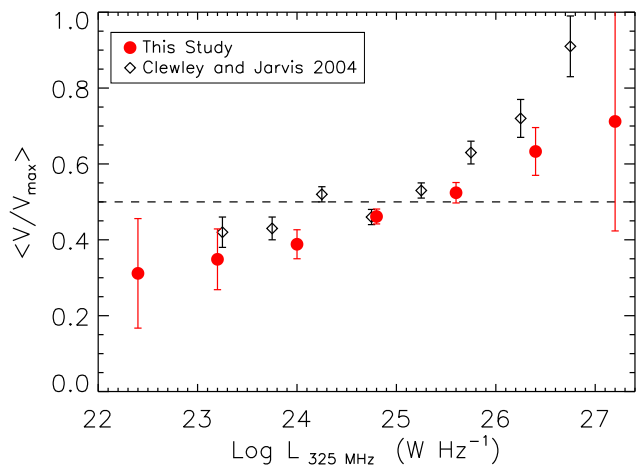
Figure 14. The V/V_{\max} statistic as a function of the radio luminosity for AGN out to z = 0.5 for the GMRT data (red circles), compared to the results of Clewley and Jarvis 2004 (black diamonds). Errors bars are given as 1/\sqrt{12N} , as in Condon et al. (2002).
