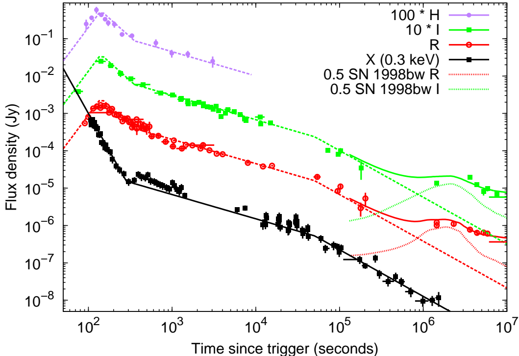
FIG. 6.— Fits to the GRB 081007 afterglow observations. The broken power-law lines with slope indices 3, -2 , -0.65 , and -1.25 for the optical/NIR (long-dashed lines), and -4 , -0.65 , and -1.25 for the X-rays (black solid line) represent the afterglow light curves. The R and I -band late observations can be interpreted as the sum (red and green solid lines respectively) of the power-law afterglow, a SN template and a host-galaxy component, here the SN is 0.5 times as bright as SN 1998bw, reported at z = 0.5295 , the host galaxy is m_R = 25.0 and m_I = 24.5 (short lines on the right). The SN template is also plotted for comparison (dotted line). The Swift /XRT X-ray light curve has been retrieved from the UK Swift Science Data Centre (Evans et al. 2009).
