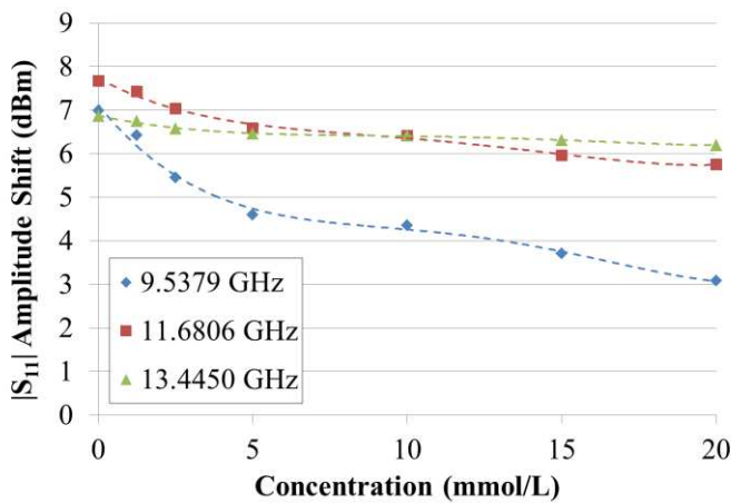
Fig. 4. Amplitude changes exhibited at 9.5379, 11.6806 and 13.4450 GHz using a cylindrical cavity resonator and varying lactate concentrations in PBS solution.
