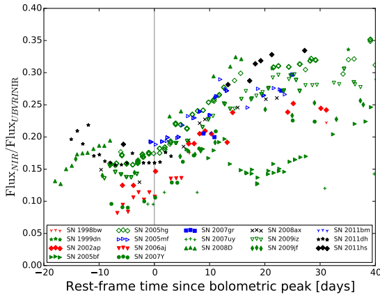
Figure 4. The ratio of NIR flux to UBVRIINIR flux. Only dates when the optical and NIR observations were coincident are included.
