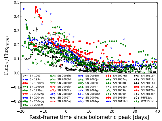
Figure 2. The ratio of the U / u' -band flux to the UBVRI flux as a function of time. Open symbols represent SNe that have not had host-galaxy extinction corrections applied. The high host extinction of PTF12os is apparent in this diagram as the U / u' flux is negligible. The temporal evolution of peculiar SN Ib 2005bf is a noteworthy feature
