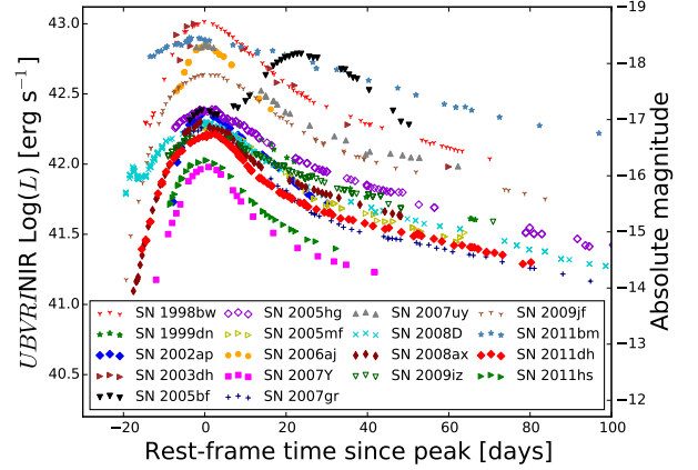
Figure 7. 18 UBVR + NIR pseudobolometric light curves constructed from optical and NIR photometry. Open symbols represent SNe without correction for host-galaxy extinction
