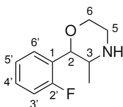
2-Fluorophenmetrazine (2-FPM)
