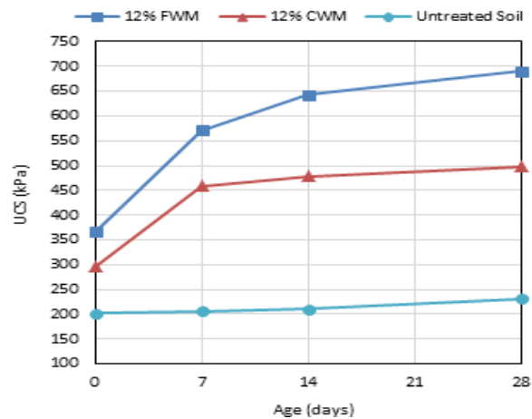
Fig. 14 UCS Development with Time of Curing
