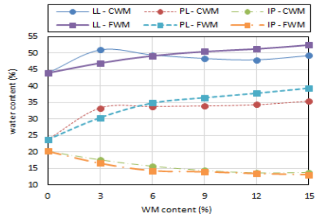
Fig. 8 Atterberg Limits for Soil Treated With CWM and FWM
