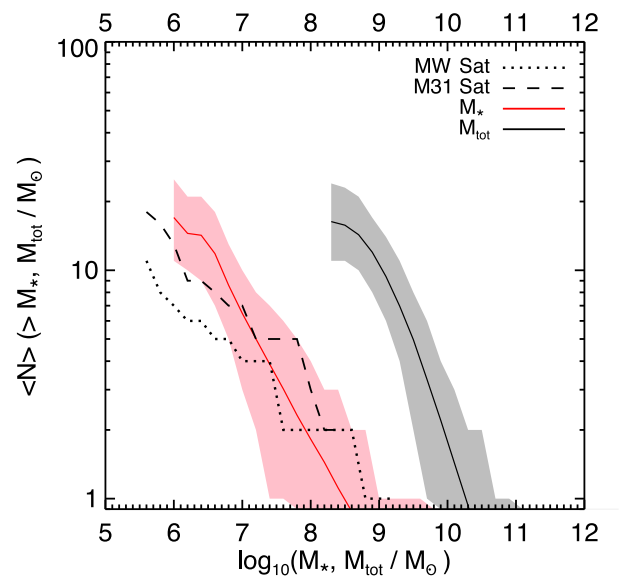
Figure A2. The mean number of luminous satellites per halo as a function of their stellar, M_* , and total, M_{\text{tot}} , masses. The shaded regions indicate the 10th and 90th percentiles scatter, while the solid lines indicate the mean value. The dotted and dashed lines show the observed stellar mass function within a distance of 300 kpc from the MW and the M31.
