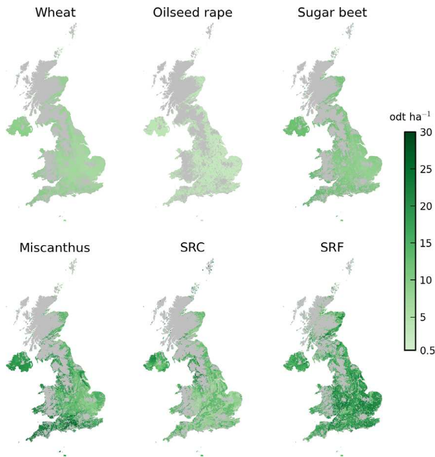
Fig. 2 Spatial distribution of modelled mean annual yield of bioenergy crops as \text{odt ha}^{-1} \text{yr}^{-1} (where odt is oven dry tonnes) in the 2030s under the UKCP09 medium emissions climate scenario. Miscanthus , SRC and SRF yields were obtained from simulations using the models MiscanFor, ForestGrowth SRC and ESC-CARBINE, respectively. Defra yield statistics from 2000 to 2008 were used to establish baseline yield values for wheat, OSR and sugar beet, which were then adjusted for future climate using the Miami model (see text).
