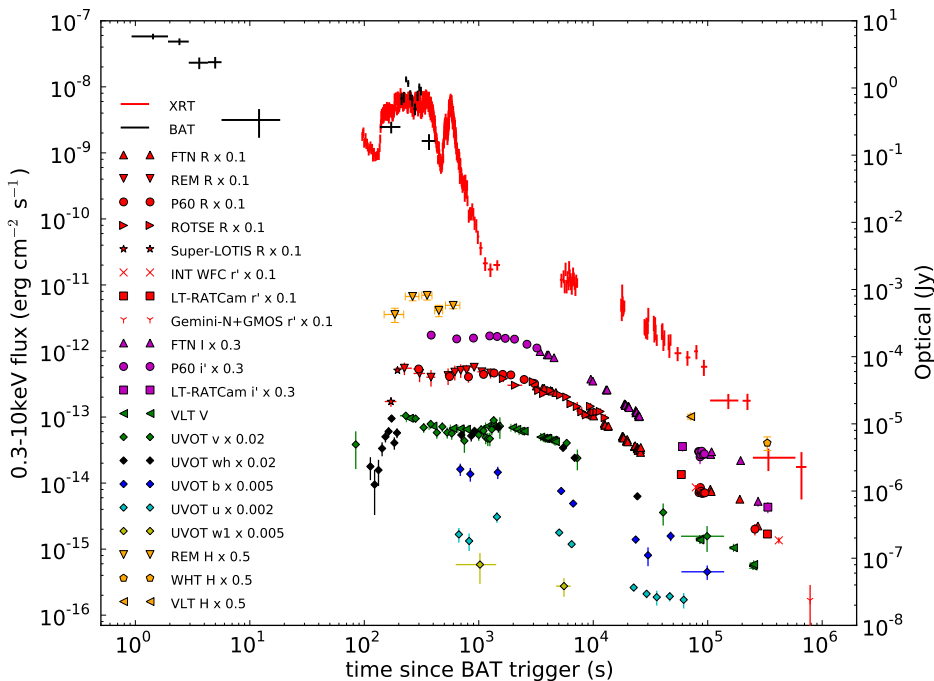
Figure 3. \gamma -ray to near IR light curves for GRB 080310, showing the energy bands used to observe the GRB and the instruments used to take the measurements. Data have been scaled from their actual values for viewing purposes.
