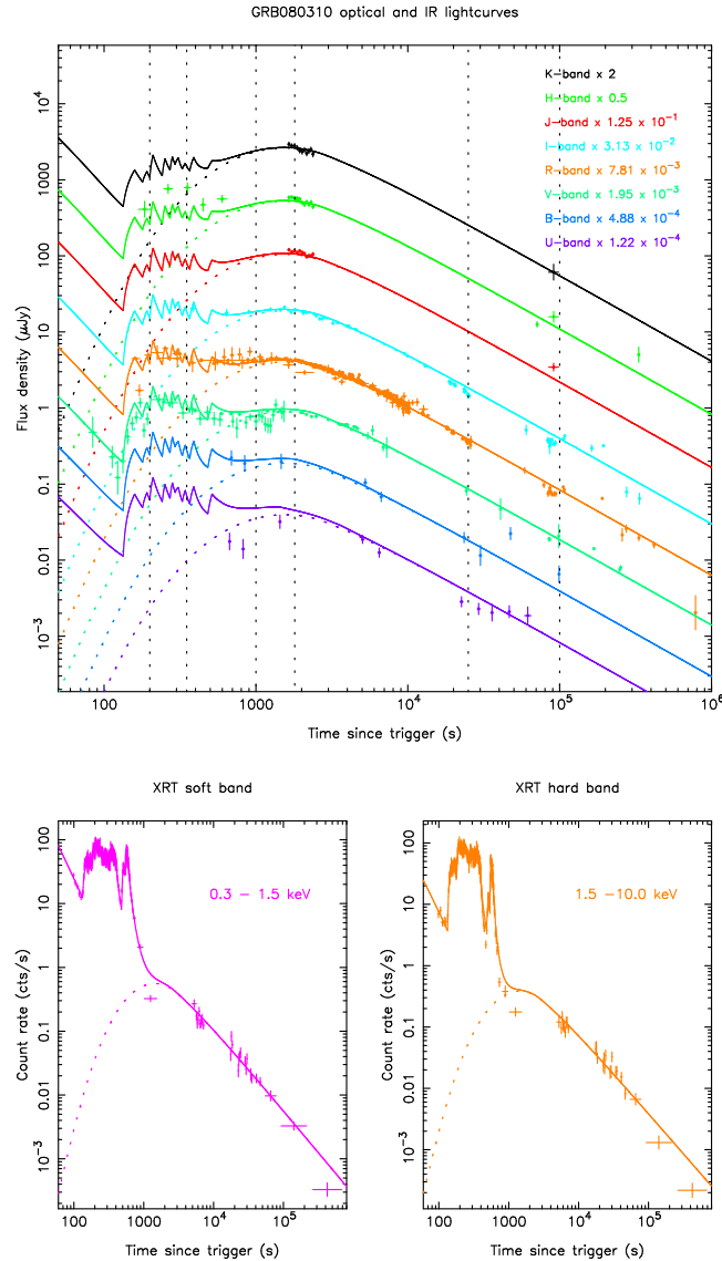
Figure 10. Simultaneous fit to optical, IR and XRT data, in which the early time optical and IR are fitted by the prompt emission. Top panel: Optical and IR bands fitted with low energy break ( K , H , J , I , R , V , B and U bands). Bottom left: XRT soft band fit. Bottom right: XRT hard band fit. E_a = 0.3 keV, p_a and d_a are allowed to float (producing a value of d_a = -1.01 ) and the afterglow parameters ( T_r , T_a , \alpha_a and F_a ) are also fitted. The reduced \chi^2 for this fit is 2.43 with 1,642 degrees of freedom.
