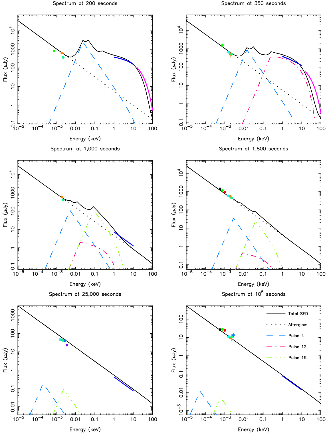
Figure 9. SEDs for fiducial times in the light curve of GRB 080310 using the afterglow model to fit the early time, low energy emission. Prompt pulses are included with a bulk value of p_a = 2.5 . The solid line is the total SED and the dotted line is the contribution from the afterglow component. Pulses 4, 12 and 15 are also shown by the dashed and dotted lines as outlined in the key shown in the bottom right panel. These are included as examples to show the evolution of some of the longer lasting pulses in the fit. The colours of the data points follow the same scheme as that used in the light curves, with the BAT and XRT data being represented by lines which extend along their entire coverage.
