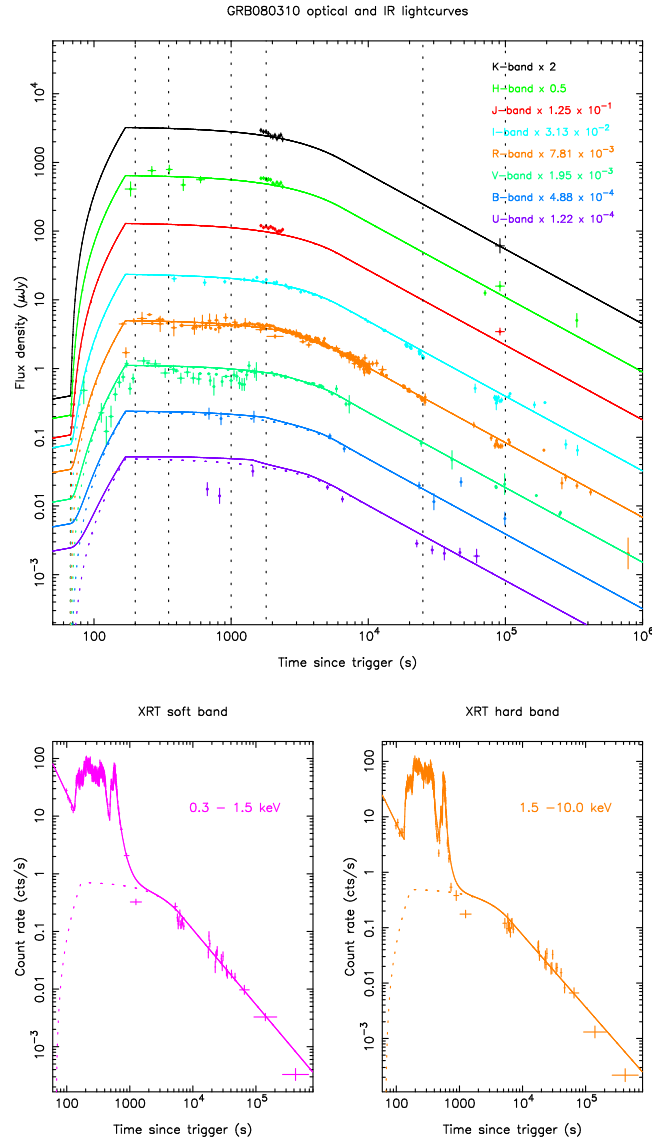
Figure 8. Simultaneous fit to optical, IR and XRT data, in which the early time optical and IR are fitted by the afterglow emission. Top panel: Optical and IR bands fitted with low energy break ( K , H , J , I , R , V , B and U bands). Bottom left: XRT soft band fit. Bottom right: XRT hard band fit. The afterglow parameters are fitted, as are values for d_a , whilst E_a = 0.3 keV and p_a has been set to \frac{5}{2} . Coloured dashed lines show the afterglow component in each band. The reduced \chi^2 for this fit is 2.44 with 1,642 degrees of freedom.
