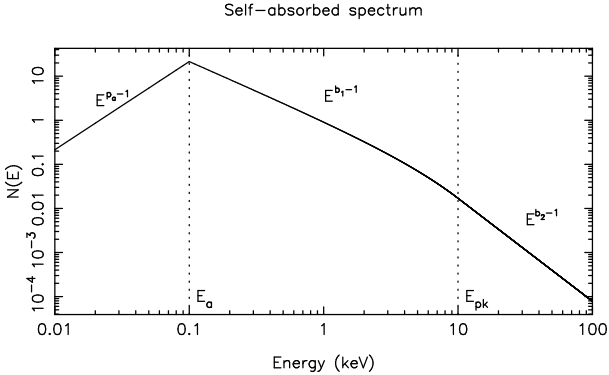
Figure 7. Example modified spectrum including additional spectral break.
