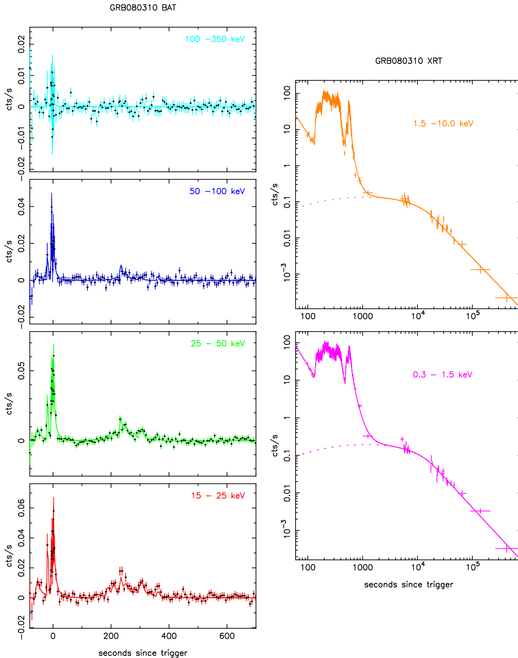
Figure 5. BAT and XRT data, showing the fitted Willingale et al. (2010) model. Left panels: BAT bands (Top to bottom: 100-350 keV, 50-100 keV, 25-50 keV & 15-25 keV). Right panels: XRT bands (Top: XRT hard band, bottom: XRT soft band). Pulse parameters have been fixed, whilst the afterglow parameters have been fitted. Solid lines show the total fit (pulses and afterglow), whilst dashed lines show only the afterglow component to the fit.
