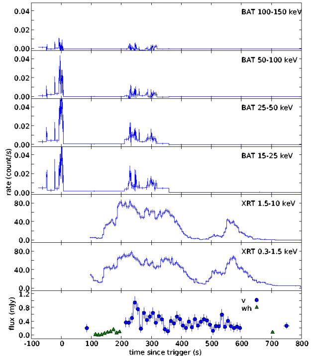
Figure 2. Swift prompt light curves from GRB 080310 in different energy bands. From top to bottom, BAT 100 – 150 keV, BAT 50 – 100 keV, BAT 25 – 50 keV, BAT 15 – 25 keV, XRT 1.5 – 10.0 keV, XRT 0.3 – 1.5 keV and UVOT v and white bands. Strictly, the count rates for BAT are per fully illuminated detector.
