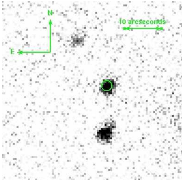
Figure 1. UVOT v -band image from T_0 + 79 s to T_0 + 1539 s. The enhanced Swift XRT position is shown (Osborne et al. 2008), with an error circle of radius 1''.4 , corresponding to the 90% confidence limit, containing the optical afterglow candidate at an average v -band magnitude of 17.49.
