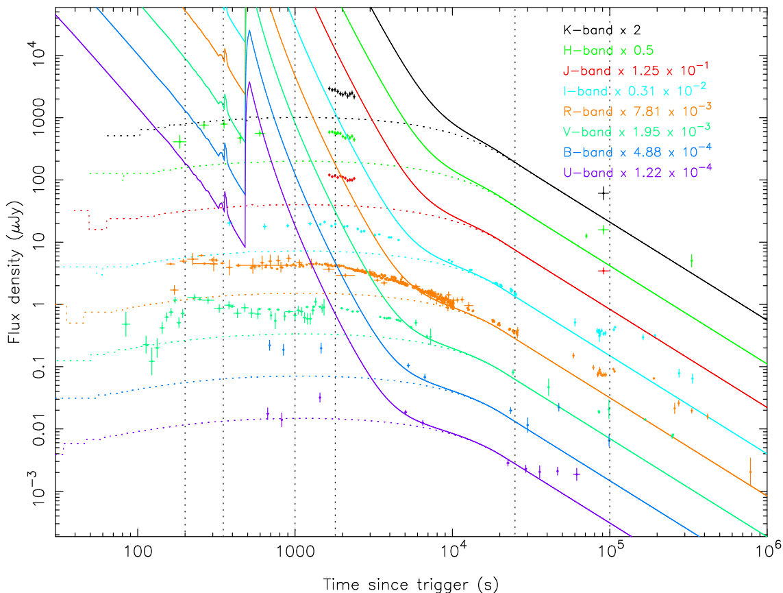
Figure 6. Optical and IR light curves obtained by extending the high energy fit to the prompt pulses and afterglow component. The spectral shape of the pulses is assumed to be a Band function extrapolated back to the optical and IR data ( K , H , J , I , R , V , B and U bands). Vertical dashed lines denote times of interest later discussed, at which the SEDs are considered in more detail. The coloured dashed lines show the afterglow component to the extrapolation for each band.
