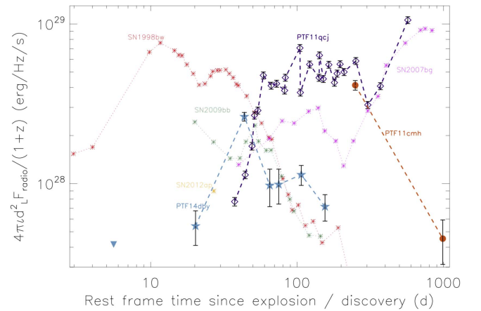
Figure 5. BL-Ic SNe in our sample with radio detections: PTF11cmh (orange dots); PTF11qej (purple diamonds; Corsi et al. 2014); and PTF14dby (blue stars). We compare these non-relativistic / CSM-interacting SNe with the light curves of the GRB-SN 1998bw (red asterisks; Kulkarni et al. 1998), of the relativistic BL-Ic SN 2009bb (green asterisks; Soderberg et al. 2010), of the CSM-interacting BL-Ic SN 2007bg (magenta asterisks; Salas et al. 2013), and of the relativistic SN 2012ap (yellow asterisk; Chakraborti et al. 2015). As evident from this comparison, the non-relativistic and CSM-interacting BL-Ic peak at later timescales than the relativistic ones.
