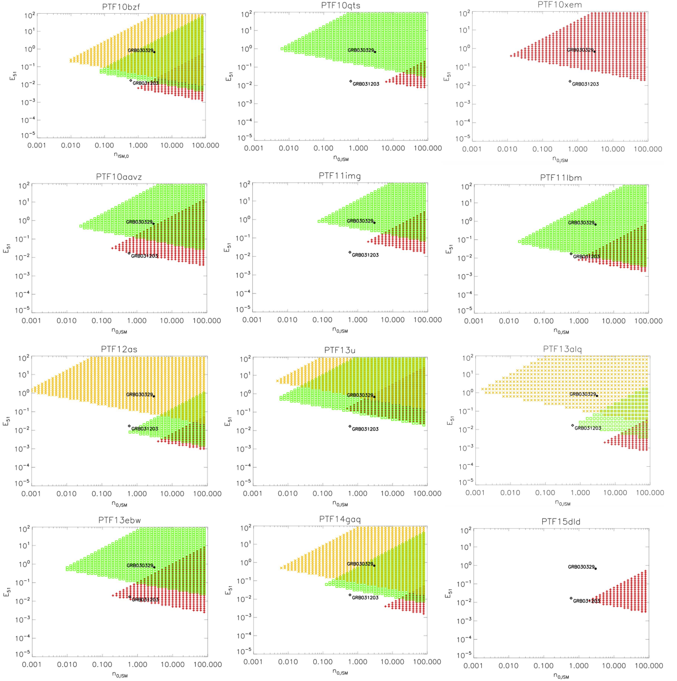
Figure 6. Regions of the energy ( E_{51} )–density ( n_{0,ISM} ) parameter space excluded by our VLA upper limits. For each SN in our sample, red, green, and yellow correspond to different observations. Specifically, for each SN, we use red for the constraints derived from the first epoch of observations, green for the second epoch (if observed twice; see Table 3), and yellow for the third epoch (if available; see Table 3).
