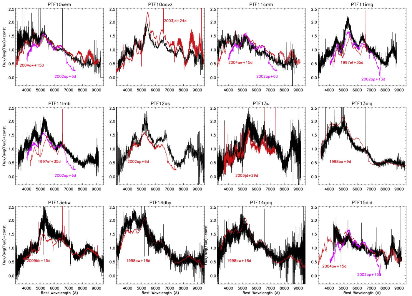
Figure 2. Spectra of the SNe BL-Ic in our sample (black) compared to the spectra of the hypernova SN 1997ef (Iwamoto et al. 2000; Branch 1999) epoch calculated since 1997 November 15), of the GRB-associated BL-Ic SN 1998bw (epoch calculated since 1998 April 25; Patat et al. 2001), of the BL-Ic SN 2002ap (epoch calculated since 2002 January 28; Gal-Yam et al. 2002; Mazzali et al. 2002), of the BL-Ic/hyper-energetic and asymmetric SN 2003jd (epoch calculated since 2003 October 21; Mazzali et al. 2005; Soderberg et al. 2006b; Valenti et al. 2008), of the Ic/BL-Ic SN 2004aw (epoch calculated assuming an explosion date of \approx 15 days before maximum; Taubenberger et al. 2006), and of the relativistic BL-Ic SN 2009bb (epoch calculated since 2009 March 19; Soderberg et al. 2010; Pignata et al. 2011).
