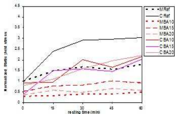
Fig. 15. Evolution of normalized static yield stress with resting time for mortars and concretes with coal bottom ash using HRWR= 0.4%.
