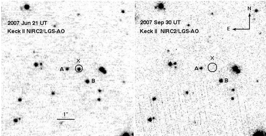
FIG. 9.— K -band image of the field of Swift J195509.6+261406 obtained with NIRC-2 imager behind the Keck II Laser Guide Star (LGS) system on 2007 June 21 ( left ) and 2007 September 30 ( right ). The 2\sigma error circle of the optical transient (taken from our LRIS imaging) is shown as a black circle overlaid on the LGS image. Clearly we can identify the object marked by the cross as the NIR counterpart of Swift J195509.6+261406.
