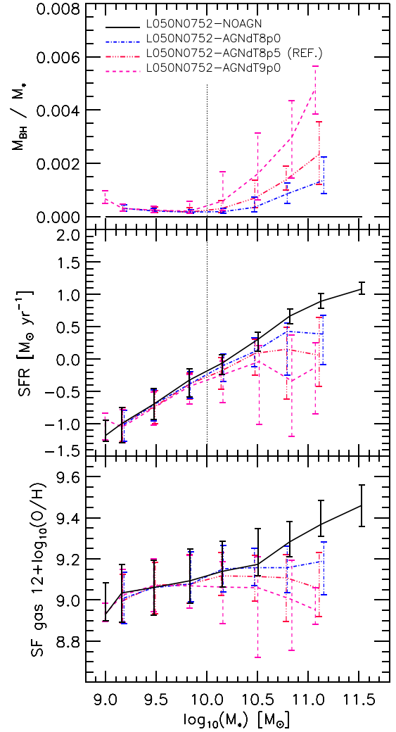
Figure 3. Simulated M_* - M_{\text{BH}}/M_* (upper panel), M_* - \text{SFR} (middle panel) and M_* - \text{O}/\text{H}|_{\text{SF,gas}} (lower panel) relations at z = 0 for different models. Results obtained from simulations ‘L050N0752’ with different AGN feedback parameters are presented: NOAGN (AGN feedback suppressed entirely), AGNdT8 ( \Delta T_{\text{AGN}} = 10^8 K), reference model ( \Delta T_{\text{AGN}} = 10^{8.5} K) and AGNdT9 ( \Delta T_{\text{AGN}} = 10^9 K). Note that AGN effects set in above M_* \sim 10^{10} M_\odot (dashed vertical line).
