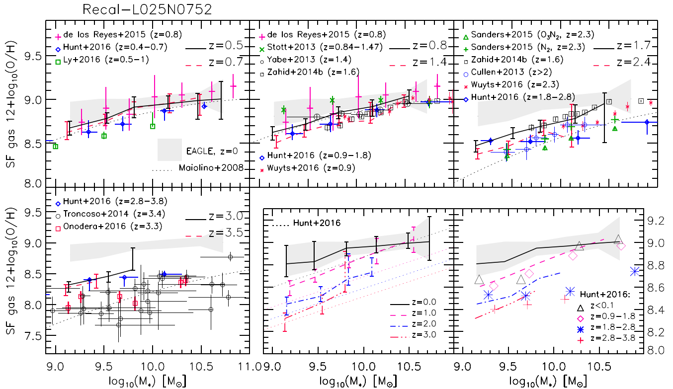
Figure 2. Large panels: Simulated M_*\text{-O/H}|_{\text{SF,gas}} relation at different z . Curves depict the median relation and error bars the 25th and 75th percentiles corresponding to simulation Recal-L025N752. Different observational results at z close to simulations are shown as symbols with error bars. Fitted relations to observations given in Maiolino et al. (2008) are represented with dotted lines. Small left-hand panel: Comparison between simulation results (curves with error bars) and fitted relations given in Hunt et al. (2016) at z = 3, 2, 1 and 0 (from bottom to top, dashed lines). Small right-hand panel: Comparison between simulation results (curves) and observed median relations at different z reported by Hunt et al. (2016) (symbols). In all cases, observed data were renormalized so that the observed local MZR considered by each author agrees with simulation results at M_* \approx 10^{10.5} M_\odot at z = 0 (see the text for details). As a reference, the area enclosed by the 25th and 75th percentiles corresponding to the simulation at z = 0 is reproduced in all panels as a grey shadow.
