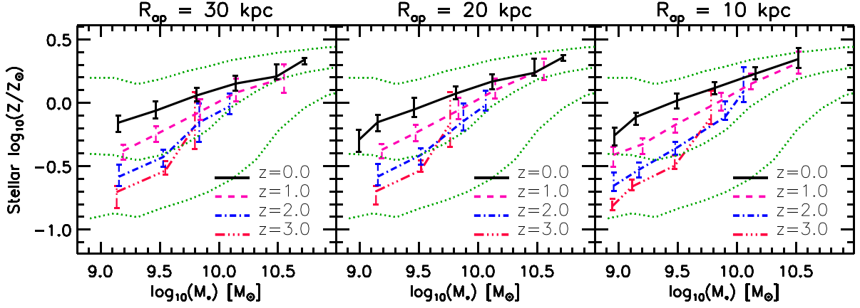
Figure A2. M_* - Z_* relation at different z for Recal-L025N0752 simulations. We compare results obtained by using different aperture radii, R_{\text{ap}} : 30 kpc (left-hand panel), 20 kpc (middle panel) and 10 kpc (right-hand panel). The simulated relations are shown as curves with error bars, depicting the median relation with the 25th and 75th percentiles. For reference, observational data at z \approx 0 from Gallazzi et al. (2005) are shown as green dotted lines and indicate the median relation and 16th and 84th percentiles. We assumed Z_{\odot} = 0.0127 (Wiersma et al. 2009b) and re-scaled observational data accordingly.
