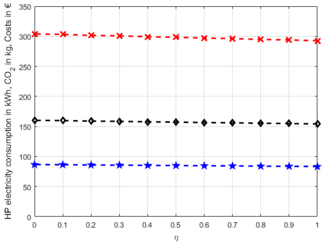
Fig. 9: Heat pump electricity energy consumption (broken red curve) in kWh, CO 2 equivalent emission (broken black curve) in kg and electricity costs (broken blue curve) in Euro as functions of heat recovery efficiency based on Fig. 8(b).
