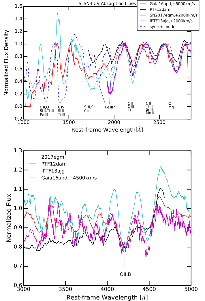
FIG. 5.— The normalized spectra in comparison with the model spectrum (blue dashed line) generated by Quimby et al. (2017) using syn++ code (Thomas et al. 2011). To align the spectral features, we redshifted the spectra by the indicated velocities. The shifts are generally different for UV and optical spectra for the same SLSN-I.
