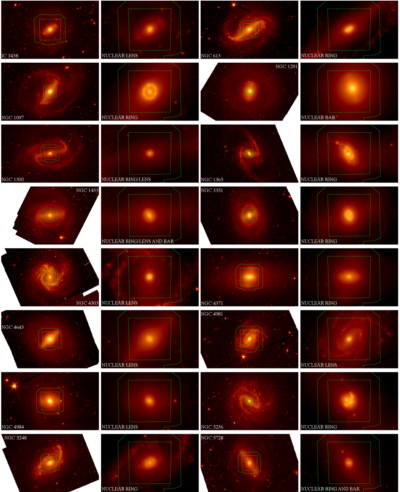
Figure 1. S^4G images at 3.6\mu\text{m} of all galaxies in the current TIMER sample. For every galaxy we show an image that includes most of the major disc, as well as an image that focuses on the area covered by our MUSE pointing. The MUSE field is represented by the inner trapezoid in green with \approx 1' on a side. The area between that and the outer polygon in green was used by the Slow-Guiding System during the exposures whenever it includes suitable point sources. North is up, east to the left.
