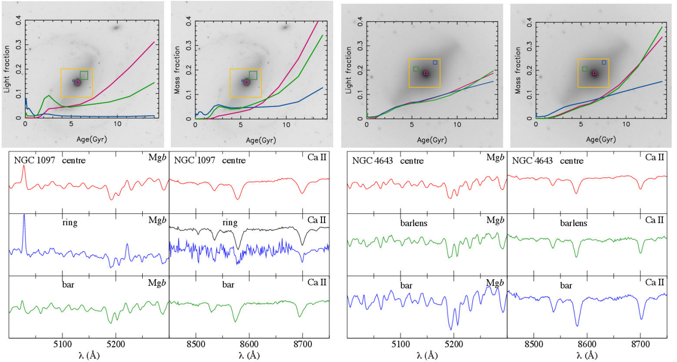
Figure 6. Top row: Star formation histories in different regions of NGC 1097 (left panels) and NGC 4643 (right panels) weighted by both luminosity and mass, as indicated. These are built from the combined spectra within each region. In each panel, our MUSE field is the yellow square overlaid on a S^4G 3.6\mu\text{m} image. Selected regions of the galaxies are shown within the different coloured rectangles, and their corresponding star formation histories are described by the lines with the same colour. These star formation histories correspond to the fraction of the stellar light (left) or mass (right) within each region as a function of stellar age. Bottom panels: For both galaxies we show the combined MUSE spectra from the three different regions (with the same colour coding) in the spectral regions around the Mgb feature and the CaII triplet, as indicated. Note that the CaII triplet region in the spectrum from the nuclear ring in NGC 1097 is heavily affected by Paschen lines, since this region coincides with a spot with very intense star formation and elevated dust content (see Cenarro et al. 2001). The spectrum shown in black in the corresponding panel is taken from a region in the immediate vicinity and with the same size, and it does not show this effect.
