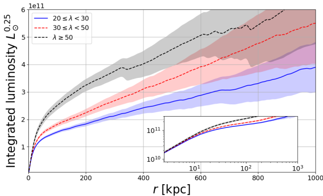
FIG. 15.— Integrated ICL luminosities at different radii of clusters in different richness ranges. The inset figure shows the same plot but with log scaling. The integrated ICL luminosities appear similar within \sim 30 kpc regardless of cluster richness. As the distance increases, richer clusters contain more ICL, which means that the ICL dependence on cluster richness is mainly driven by the diffuse light outside the cores of the CGs.
