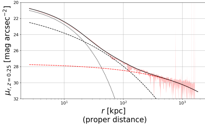
FIG. 10.— The ICL+CG light profile can be approximated with three Sersic components (black solid line): a core disk component that is dominant within 10 kpc (dotted line), a bulge component that is dominant between 30 and 100 kpc (dashed line), and a diffuse component that is dominant outside 200 kpc (red dashed line).
