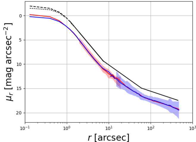
FIG. 7.— Extended PSF of DECAM+Blanco 4m in the g - and r - bands. The PSF is constructed by piecing together images of 19th, 14th, and 8th magnitude stars, each of which samples the PSF at good S/N (without saturating) at a different range of radii. g - and r - band average profiles are shown with solid blue and red curves, respectively. The shaded red curve at 10'' < r < 20'' is derived with 14th magnitude r -band stellar images, and the shaded blue curve beyond 20'' is from 8th magnitude stellar profiles. This plot shows the profile with the central surface brightness normalized to 0 mag arcsec ^{-2} . The black curves offset above the measured profiles are fitted models containing a Gaussian (dotted line, g -band)/Moffat (dashed line, r -band) central component and then three broken power-law sections as described in the Section 4.
