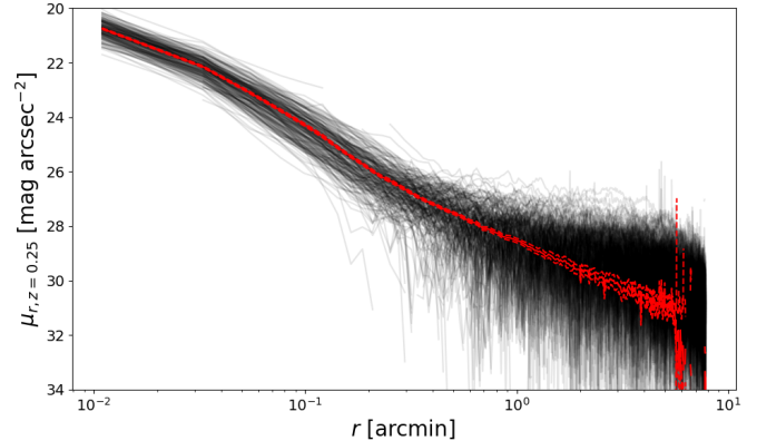
FIG. 8.— This figure shows the ICL+CG profile measurements of individual clusters (black lines) and the stacked result (red solid and dashed lines indicating the mean and the uncertainties). Stacking significantly improves the precision of cluster light profile measurement beyond 0.5 arcmin.
