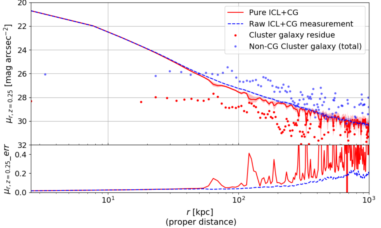
FIG. 9.— This figure shows the derived ICL+CG profiles (upper panel) and the uncertainties of the measurements (lower panel). The cluster galaxy residual (red point) is subtracted from the raw ICL+CG measurement (blue line) to derive the "pure" ICL+CG profile (red line). Uncertainties of the profiles are displayed as the shaded regions (upper panel) and also shown in the lower panel. The ICL+CG profiles are measured with high S/N to 1 Mpc, although the subtraction of cluster galaxy residual introduces significant noise (poisson noise) into the "pure" ICL profile.
