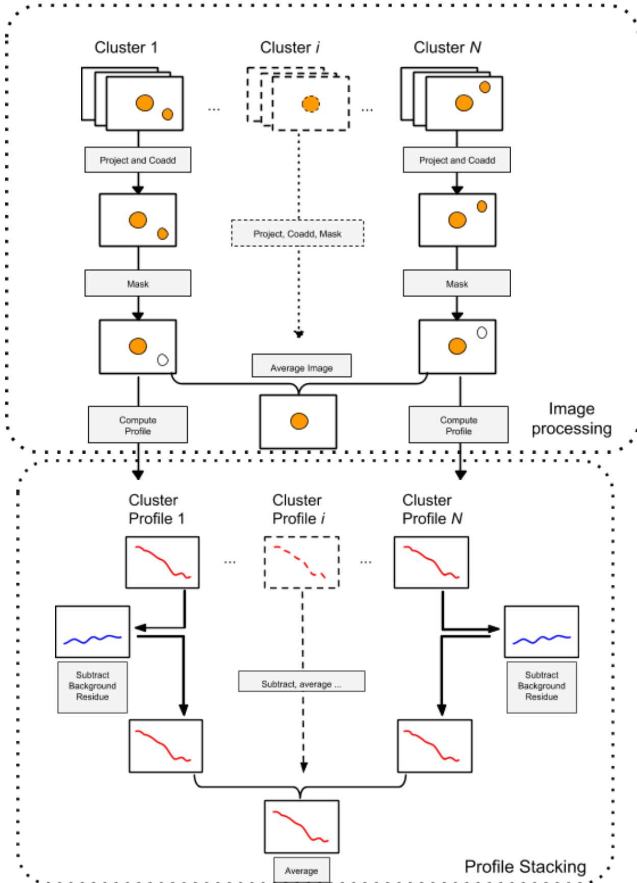
FIG. 2.— The ICL analysis in this paper starts with DES single exposure images. The single exposure images are stacked, the detected objects are masked, and a raw ICL+CG light profile is derived for each cluster. These raw measurements go through a residual light subtraction process which removes residual background and cluster selection effects. The light profiles are finally averaged over all the clusters to create the stacked ICL+CG measurements.
