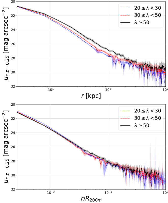
FIG. 14.— Upper panel: ICL profiles of clusters in different richness ranges. The ICL is more luminous and extended in richer systems. Lower panel: ICL profiles appear to be “self-similar”, in that after scaling with cluster radius ( R_{200m} ), the ICL profiles of clusters in different richness ranges are indistinguishable.
