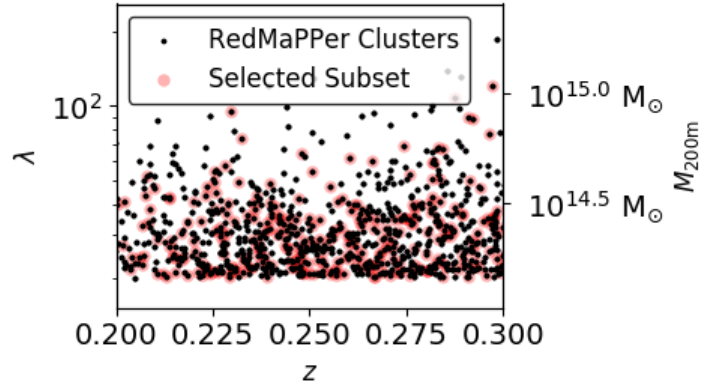
FIG. 1.— Redshifts and richnesses of the REDMAPPER clusters used in this work. The masses of the clusters are estimated from richnesses using the mass-richness relation in Melchior et al. 2017. The mean mass of the clusters studied in this paper, which pass the purging criteria in Section 2.1 (red shaded symbols, the “Selected Subset”), is 2.50 \times 10^{14} M_{\odot} .
