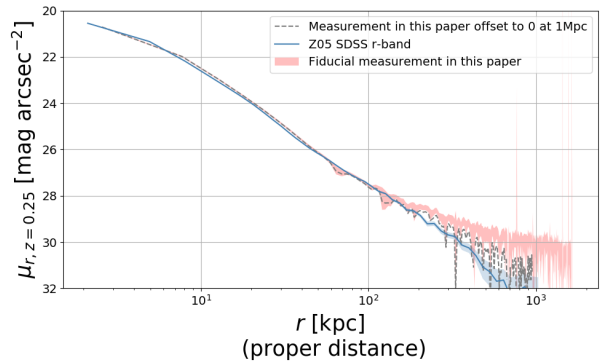
FIG. 19.— Our ICL+CG radial profile (DES r -band, red shaded region) in comparison to the measurements in Z05 (SDSS r -band, blue shaded region). Our measurements agree remarkably well with Z05 within 100 kpc, yet are much brighter than Z05 outside 100 kpc. The different background estimation methods partially explain the differences – when offsetting our ICL flux measurements to 0 at 1 Mpc (as is done in Z05), our measurement agrees better with Z05 (dashed gray line). See section 8.1 for discussions.
