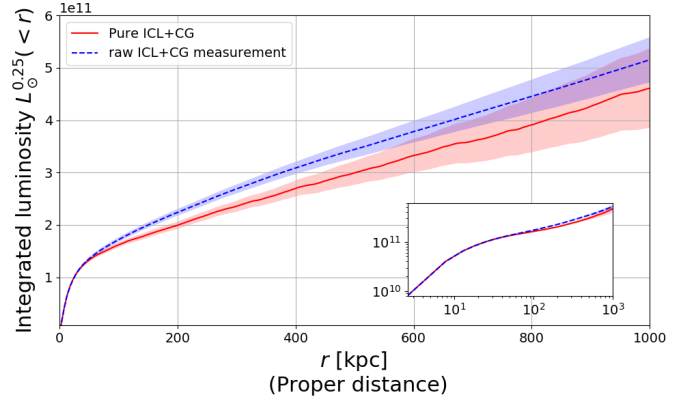
FIG. 11.— Integrated ICL+CG luminosity within different radii. The inset figure shows the same plot but with log scaling. Within \sim 30 kpc, the integrated ICL+CG luminosity steeply increases with distance because of the dominance of the CGs. The increase slows down outside \sim 30 kpc, indicating that the light distribution has transitioned into a diffuse component.
