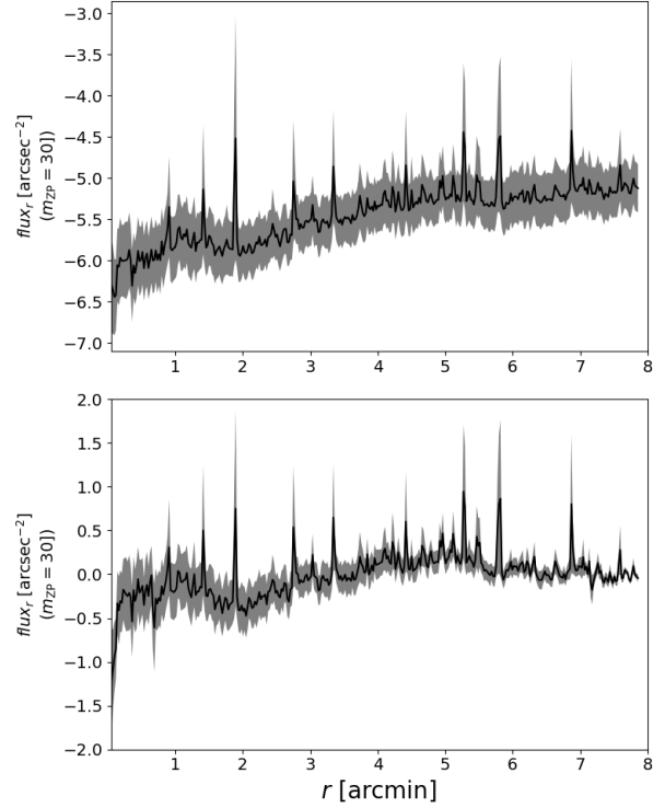
FIG. 4.— We apply our ICL detection methods to a set of random points of similar size to the cluster sample. This figure (black lines) demonstrates the effectiveness of random field subtractions in deriving the stacked light profile of random points. The upper panel shows the stacked light profile (after object masking) before subtracting the profiles of random fields. The lower panel shows the stacked light profile after subtracting random fields and the residual background. The subtraction steps reduce the correlated noise and eliminate the contamination light from cluster selection effects. In the lower panel, the stacked profile of the random points is consistent with 0, which is the evidence of unbiased measurement.
