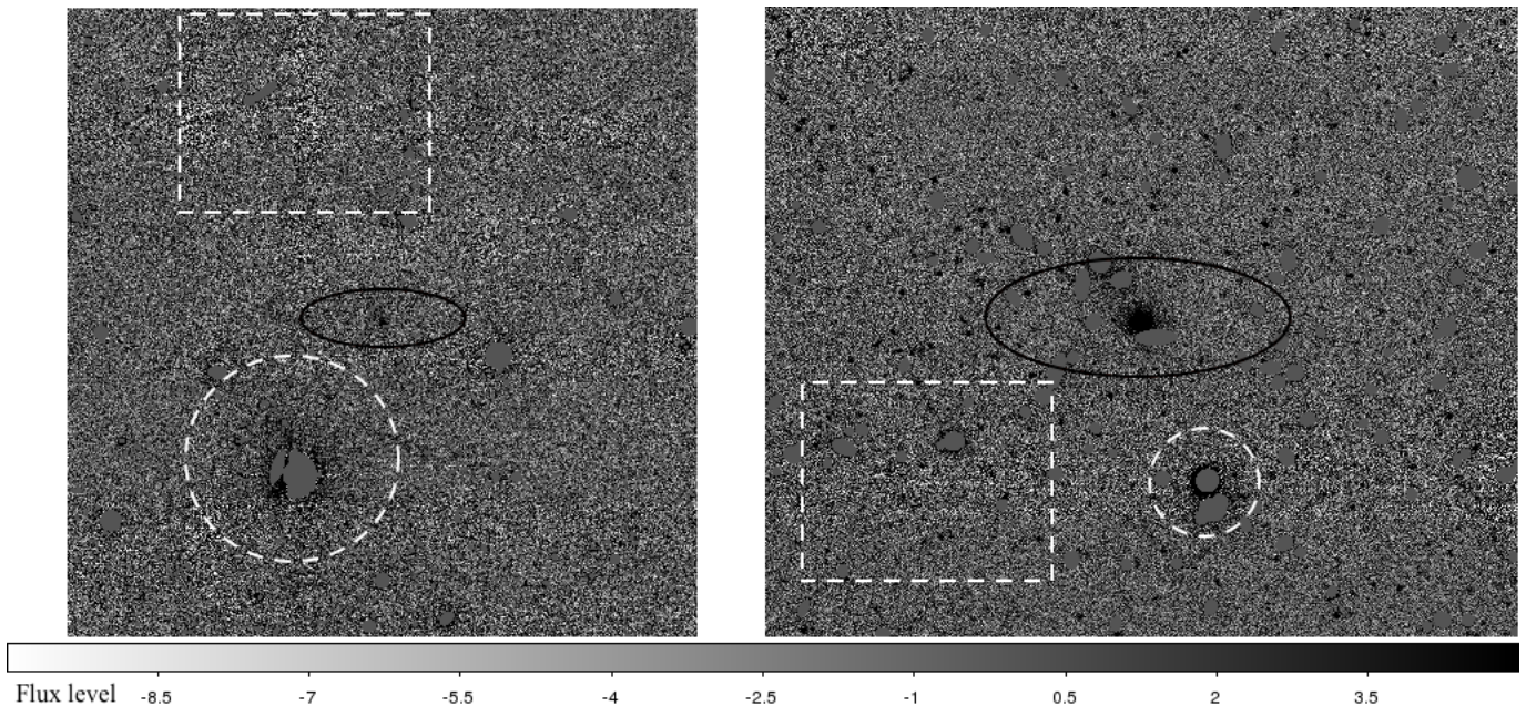
FIG. 20.— Masked r band images of one cluster in our analysis, centered on the CG. The left panel shows the whole 4000 \times 4000 pixels (1 pixel = 0.263'' ) image, and the right panel is a DS9 1/2 zoom-in of the same cluster. Bright galaxies or stars above 22.4 magnitude in i band other than the CG have been masked, but the unmasked fainter objects can be seen in the right panel. The black ellipticals indicate the CG location. The dotted circles indicate regions with sky flux discontinuities from coadding multiple single exposures. The gray bar below the image indicates the flux level while both of the images have a magnitude zeropoint of 30.
