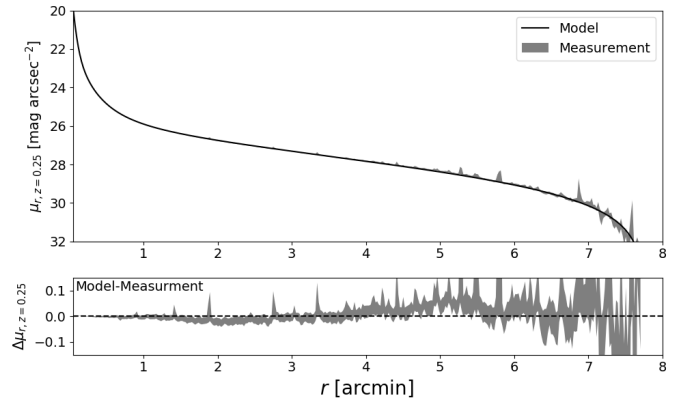
FIG. 6.— Measurement of the simulated ICL+CG profile injected at the random points. The upper panel shows the measured ICL+CG profile, and the solid line shows the injected model. The method recovers the light profile of the simulated ICL distribution out to \sim 7 arcmin from the center, at a surface brightness level of 30 mag/arcsec ^2 . The lower panel shows the residue between the measurement and the model, with the gray shaded area representing the uncertainties of the measurements.
