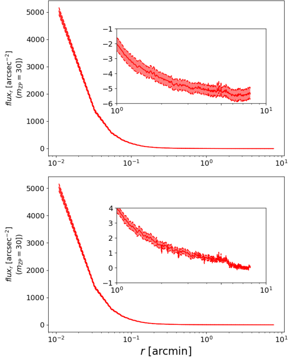
FIG. 3.— This figure demonstrates the effect of random field subtractions on the ICL+CG profile measurement. The upper panel shows the stacked cluster light profile (after object masking) before subtracting the profiles of random fields. The lower panel shows the stacked light profile of the same clusters after subtracting random fields and residual background. The insets zoom onto the profiles at large cluster radius. The subtraction steps reduce the correlated noise and eliminate the contamination light from the cluster selection effects. The effectiveness of the subtractions is more evident in the random test shown in Figure 4.
