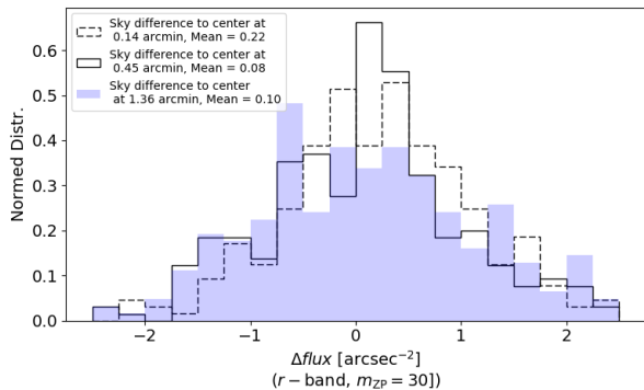
FIG. 17.— The differences in the sky level estimations between the cluster centers and locations away from the cluster centers. These differences are calculated by subtracting the sky level at a distance from the sky level at the cluster center, rescaled as the flux per arcsec 2 with a magnitude zero point of 30. See section 7.1 for discussions on the implications of this figure.
