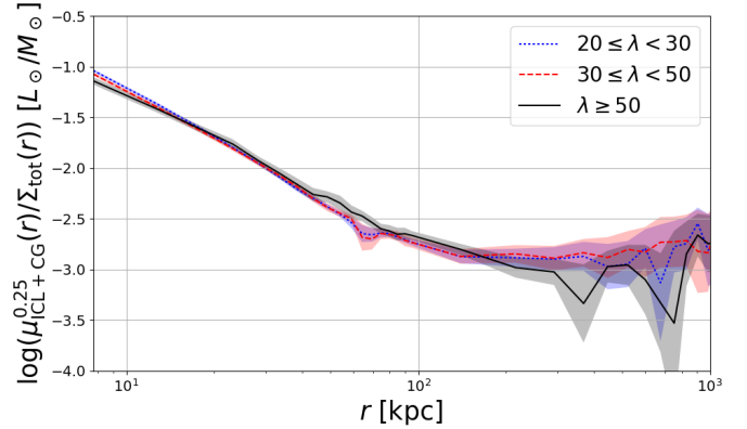
FIG. 16.— Ratios between ICL+CG luminosity and total cluster mass at different radii. Outside 100 kpc, the ICL luminosity-to-cluster-mass ratio appears flat within uncertainties, an indication that ICL luminosity traces the cluster mass distribution. Interestingly, the radial range of ratio flattening is coincident with where the ICL+CG profile transitions into a diffuse component (Figure 10). Note that the ICL+CG profiles have been rebinned by a factor of 15 outside 100 kpc from Figure 14 to reduce noise.
