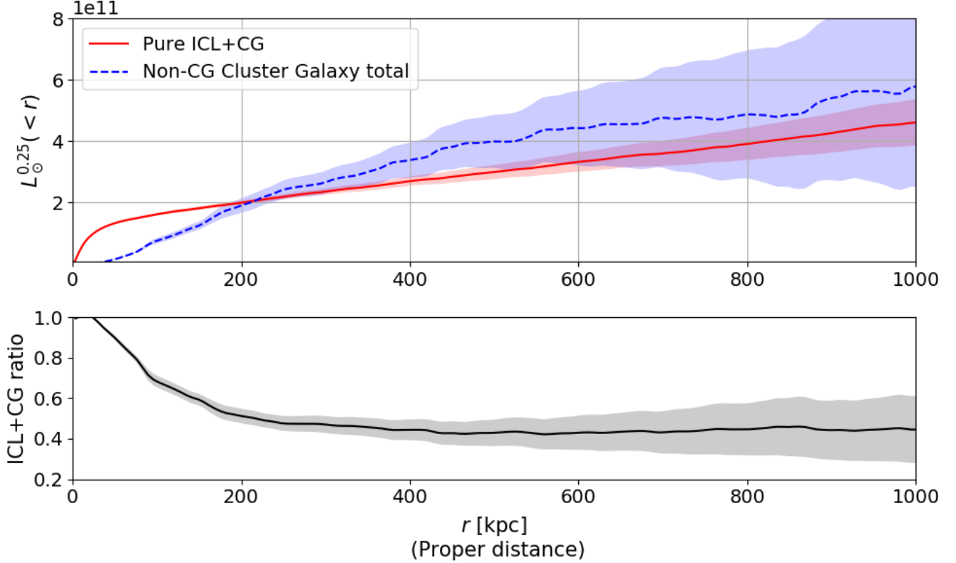
FIG. 12.— Integrated ICL+CG luminosity (red) and non-CG cluster galaxy luminosity (blue) within different radii. Within the inner 200 kpc, ICL+CG luminosity is more abundant than that of the non-CG cluster galaxies. Outside 200 kpc, the total luminosity of non-CG cluster galaxies becomes higher. Within 1 Mpc, the luminosity of ICL+CG makes up 44% (bottom panel) of the total cluster stellar luminosity computed as the sum of the non-CG cluster galaxies and the ICL+CG.
