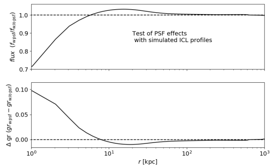
FIG. 18.— The effects of the PSF on the measurement of the flux profile (upper panel) and color profile (lower panel) of ICL+CG, tested with a simulated ICL+CG profile. We create the simulated ICL+CG profile at z = 0.25 using a combination of three Sersic models (Section 5.1), and convolve it respectively with the average DES Y3 g and r PSFs derived in Section 4. The upper panel shows the difference in flux per arcsec 2 before and after the PSF convolution in the r band. The lower panel shows the g-r color difference before and after PSF convolutions in the g - and r -bands. We find that the PSF shifts both the flux profile and the color profile, but only within the inner 10 kpc. See section 7.2 for more detailed discussions.
