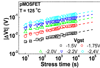
Figure 1. An example of the conventional multiple tests under different voltages for NBTI [10].
