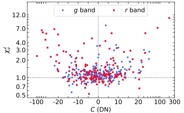
Figure 5. Distribution of \chi_{\nu}^2 and C color coded by filters ( g and r ). Note that the horizontal axis is shown with a linear scale for -20 < C < 20 and a log scale for |C| > 20 . The vertical axis is shown in a log scale. The dashed horizontal line indicates \chi_{\nu}^2 = 1 and the dashed vertical line indicates C = 0 . The median of C is -1.49 , and the median of \chi_{\nu}^2 is 1.21 .
